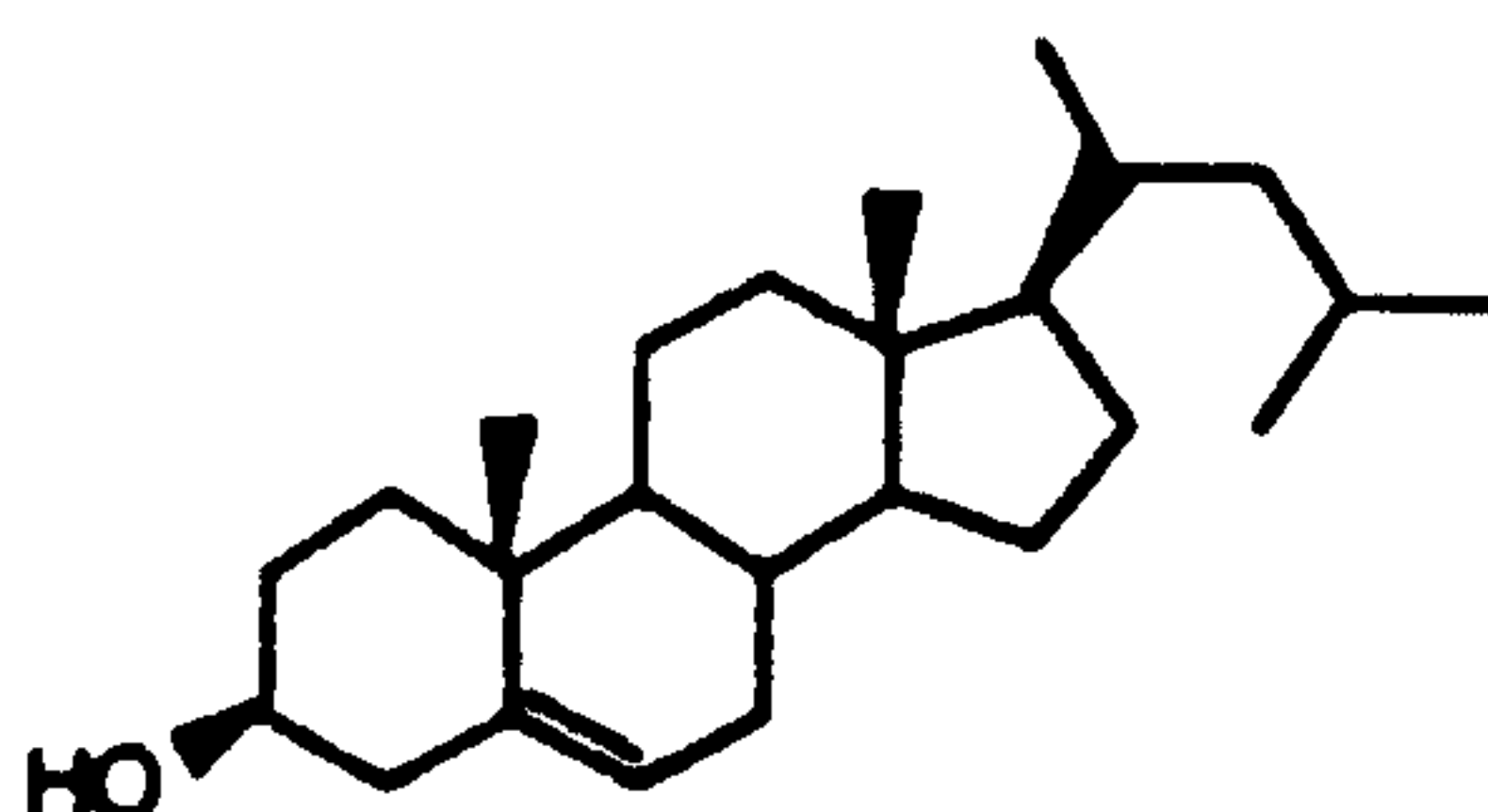
23-METHYL
