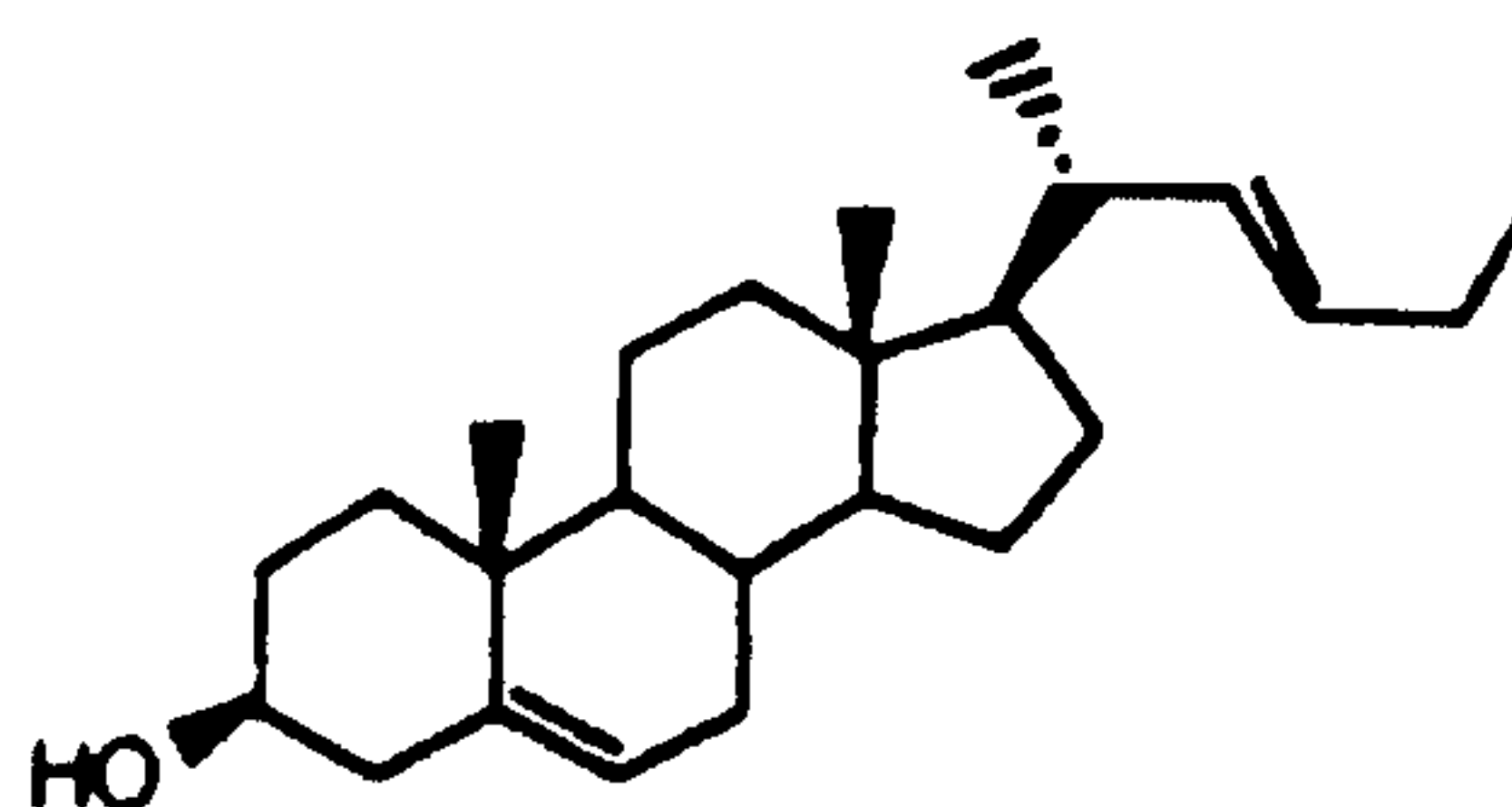
24-METHYL
