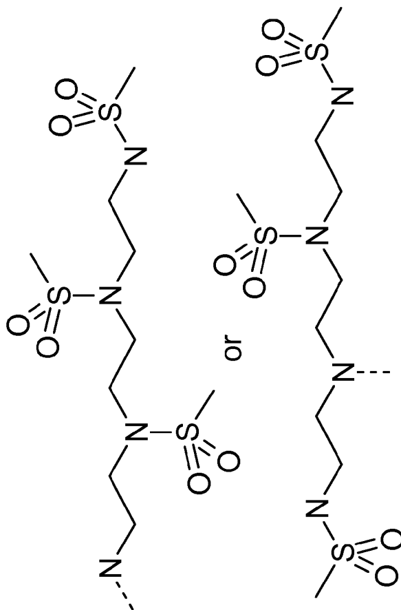
Triethylenetetramine
