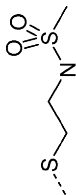
Cysteamine
