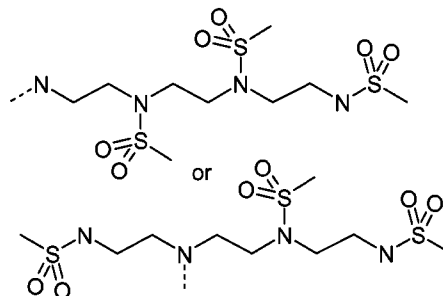
Triethylenetetramine
