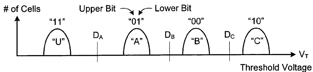
Multistate Memory (LM Gray Code)
