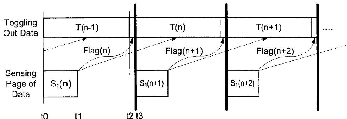
Read Caching with LM Coding
