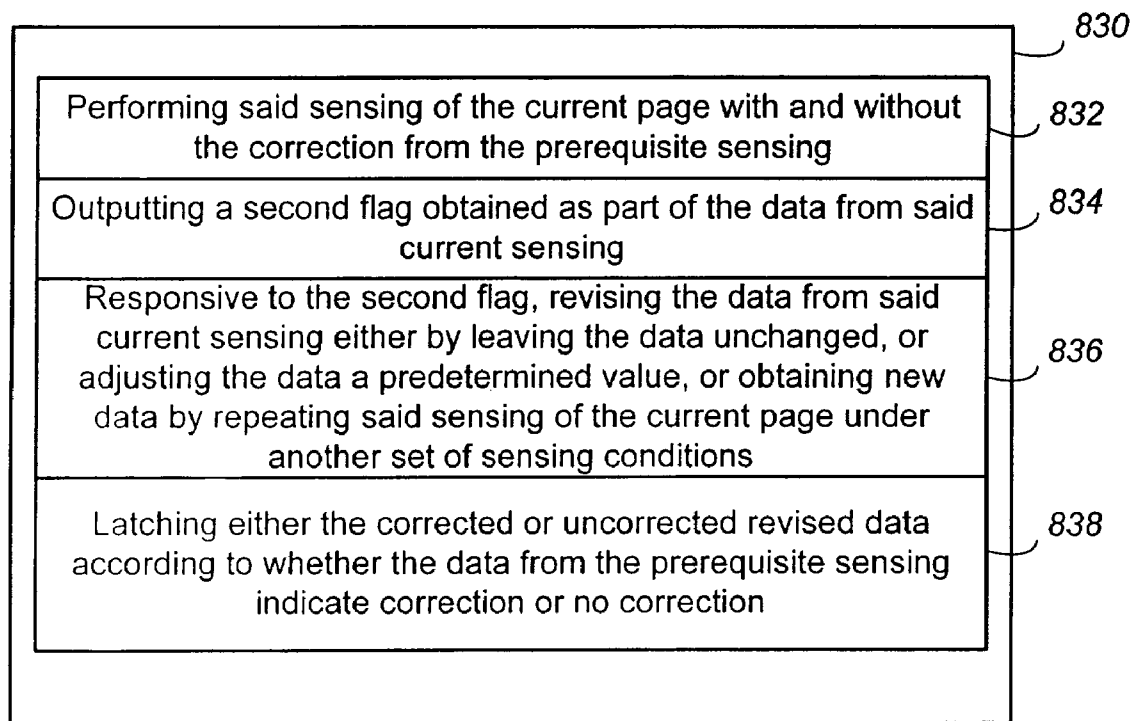
Operation of the Current Sensing
