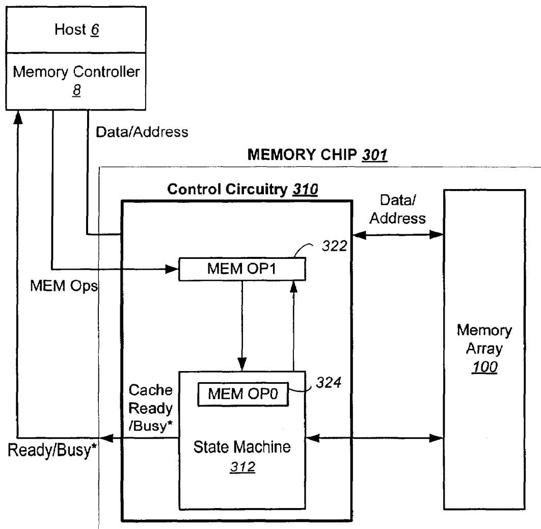
CONVENTIONAL CACHED MEMORY OPERATION
