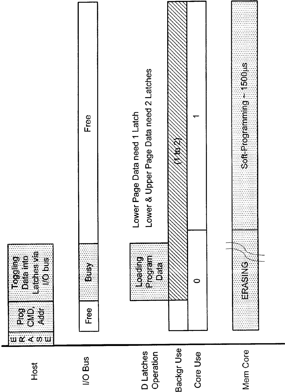
BACKGROUND PROGRAM DATA LOADING DURING ERASE PHASE
