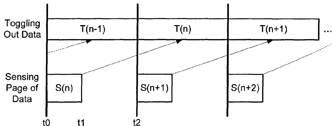
Conventional Read Caching
