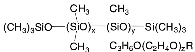
10 Formula V
