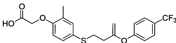
Compound 20
