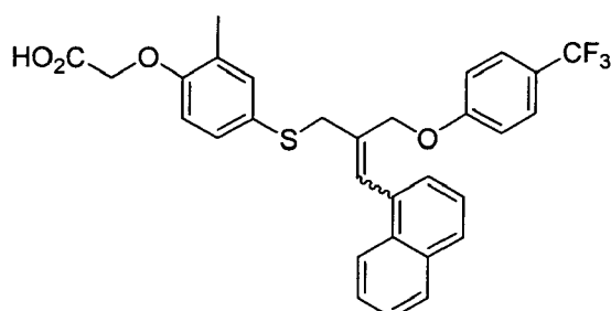
Compound 19
