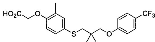
Compound 23
