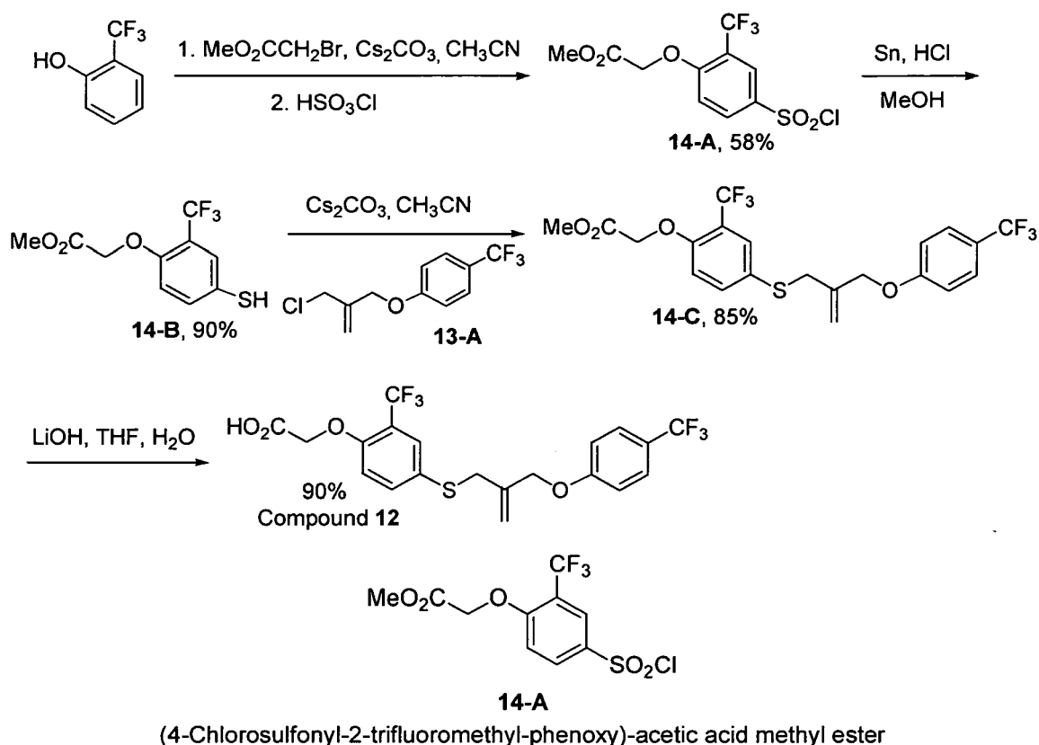
Scheme 14
