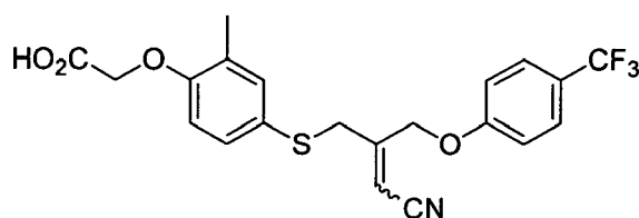
Compound 17 {4-[3-Cyano-2-(4-trifluoromethyl-phenoxy)methyl]-allylsulfanyl]-2-methyl-phenoxy}-acetic acid
