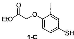
(4-Mercapto-2-methyl-phenoxy)-acetic acid ethyl ester
