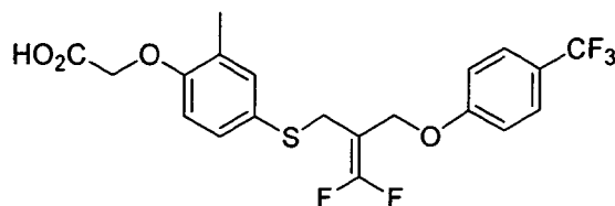
Compound 16
