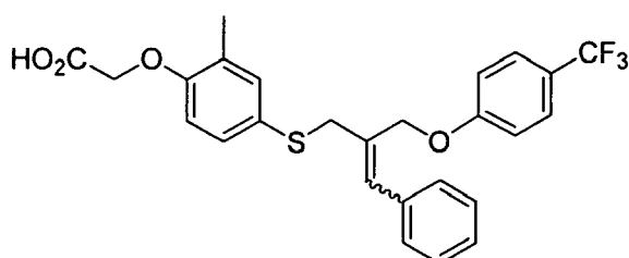
Compound 18
