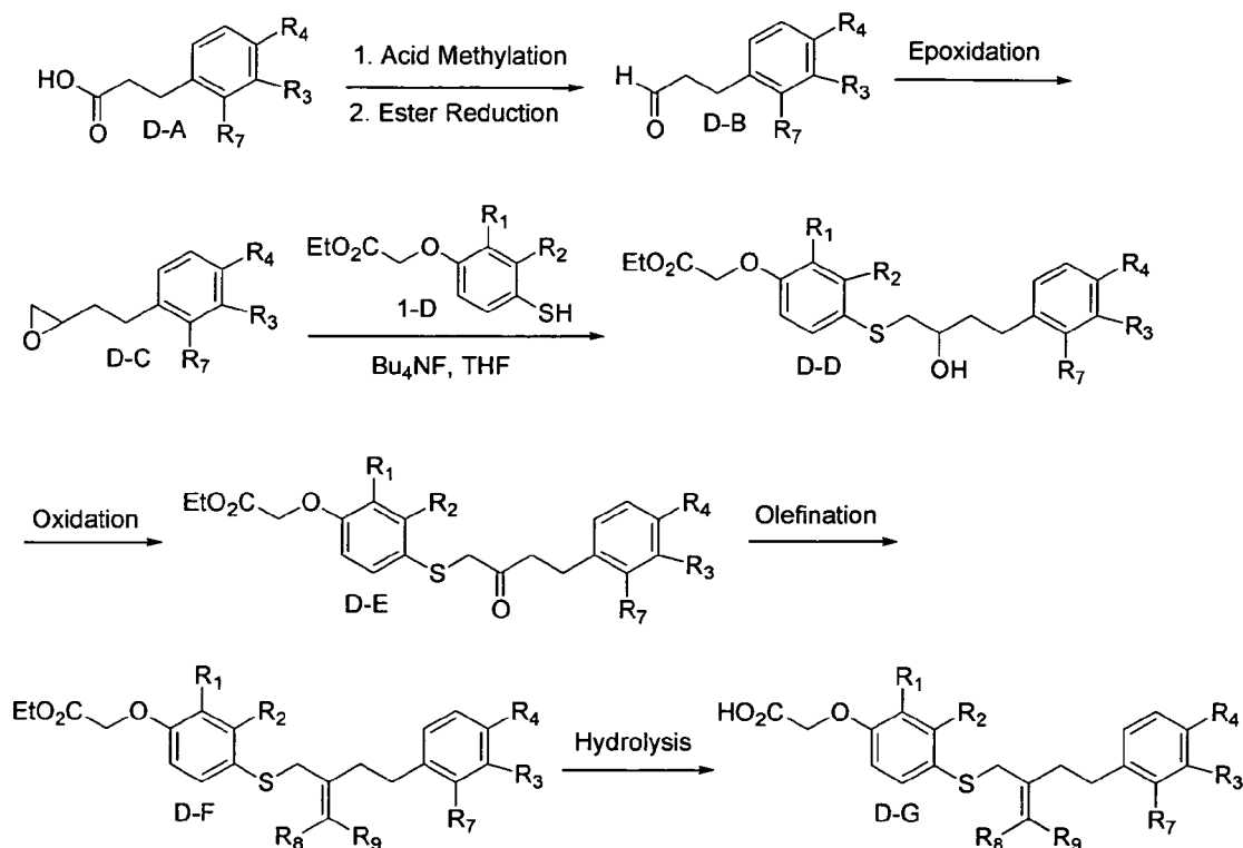
Scheme D
