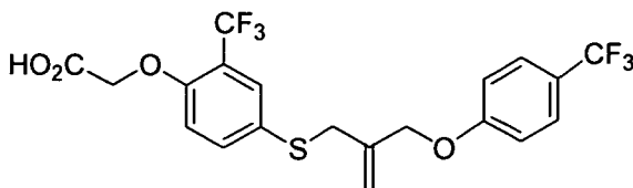
Compound 12
