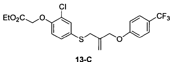
13-C {2-Chloro-4-[2-(4-trifluoromethyl-phenoxy)-allylsulfanyl]-phenoxy}-acetic acid ethyl ester
