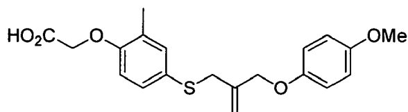
Compound 9
