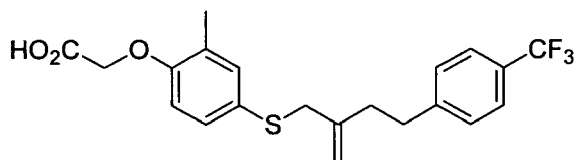
Compound 2
