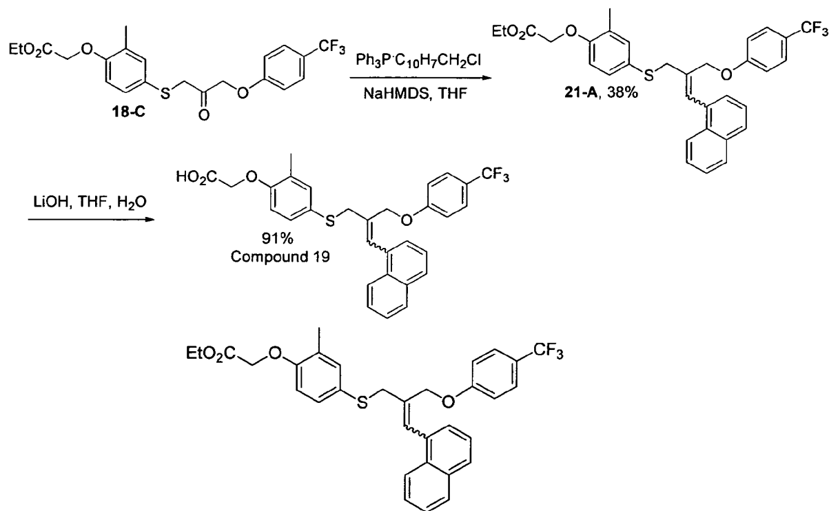
Scheme 21
