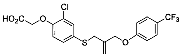
Compound 11
