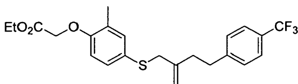
4-G
