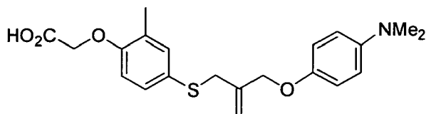
Compound 10
