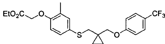
28-E
