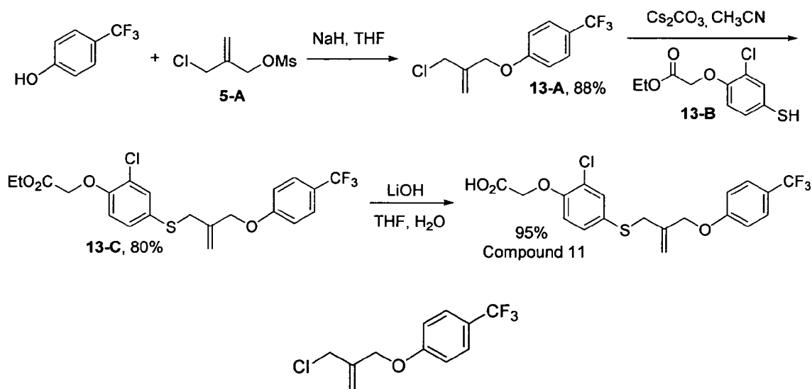
13-A 1-(2-Chloromethyl-allyloxy)-4-trifluoromethyl-benzene
