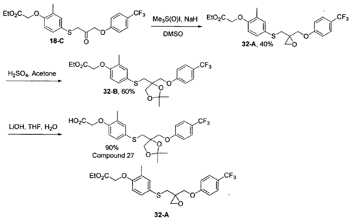
Scheme 32
