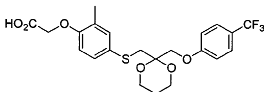
Compound 26
