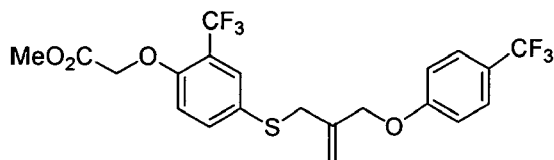
14-C
