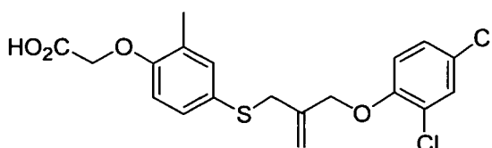
Compound 7
