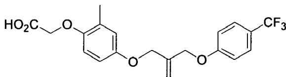
Compound 29
