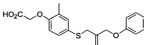
Compound 3
