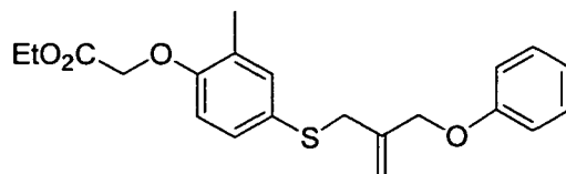
5-C
