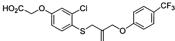
Compound 13
