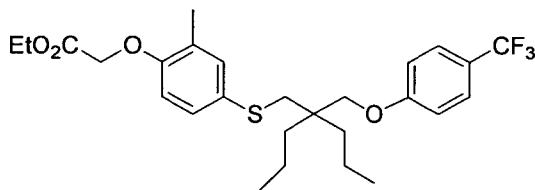
29-E
