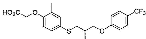
Compound 1
