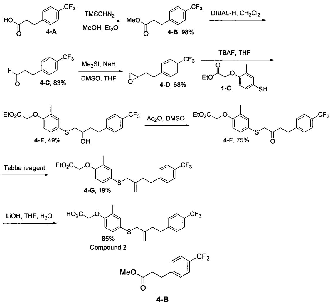
3-(4-Trifluoromethyl-phenyl)-propionic acid methyl ester
