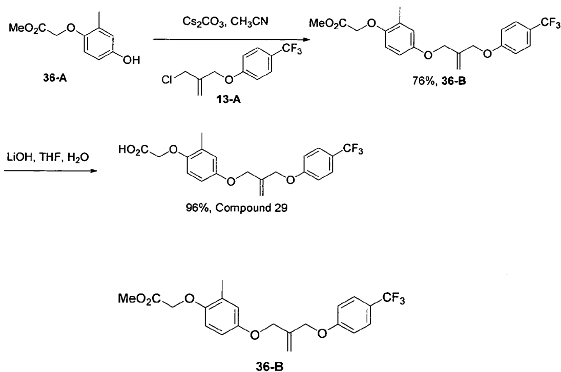
Scheme 36
