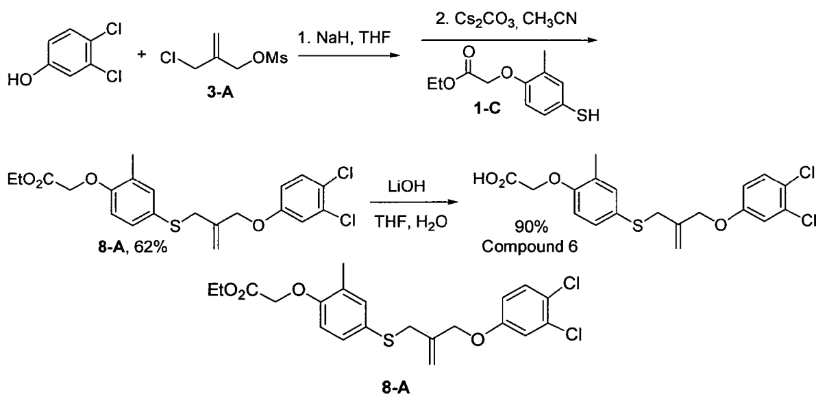
Scheme 8
