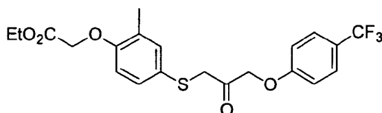
18-C
