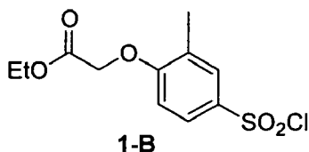
(4-Chlorosulfonyl-2-methyl-phenoxy)-acetic acid ethyl ester
