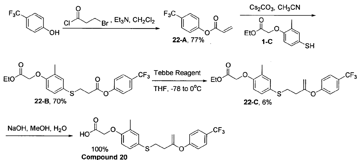
Scheme 22
