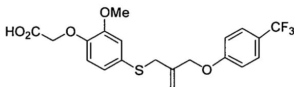
Compound 14
