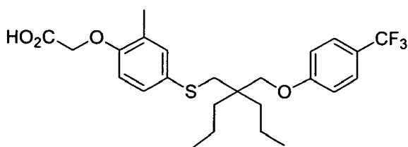
Compound 24
