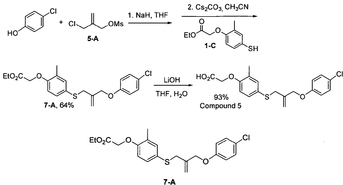
Scheme 7
