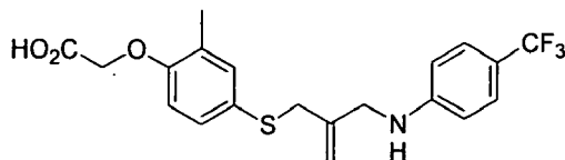
[2-methyl-4-[[2-[[[4-(trifluoromethyl)phenyl]amino]methyl]-2-propenyl]thio]phenoxy]-acetic acid
