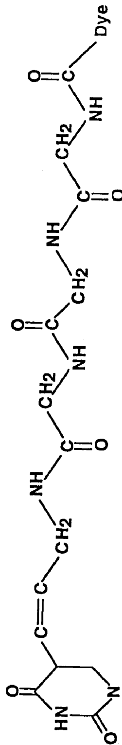
Tetraglycinyllinker
