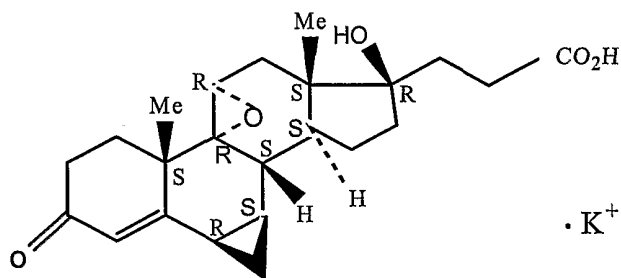
3'H-cyclopropa[6,7]pregna-4,6-diene-21-carboxylic acid, 9,11-epoxy-6,7-dihydro-17-hydroxy-3-oxo-, monopotassium salt, (6 \beta ,7 \beta ,11 \alpha ,17 \beta )-
