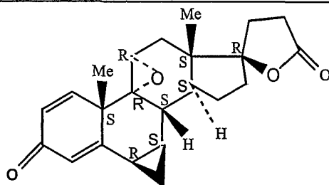
3'H-cyclopropa[6,7]pregna-1,4,6-triene-21-carboxylic acid, 9,11-epoxy-6,7-dihydro-17-hydroxy-3-oxo-, \gamma -lactone (6 \beta ,7 \beta ,11 \alpha )-
