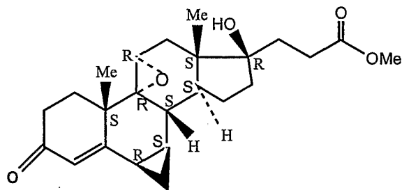
3'H-cyclopropa[6,7]pregna-4,6-diene-21-carboxylic acid, 9,11-epoxy-6,7-dihydro-17-hydroxy-3-oxo-, methyl ester, (6 \beta ,7 \beta ,11 \alpha ,17 \beta )-
