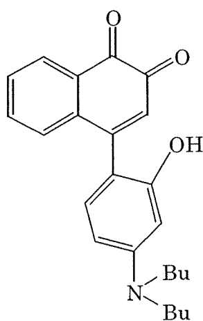
intermediate 1
