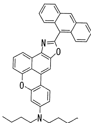
compound 8
