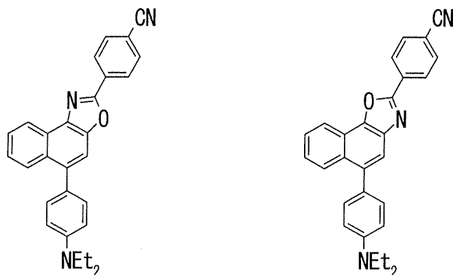
Compound 1
