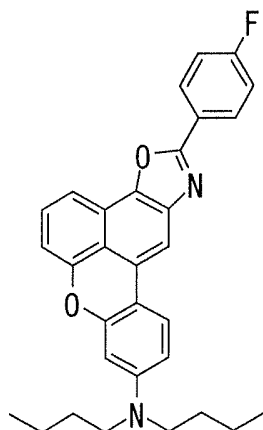
compound 15
