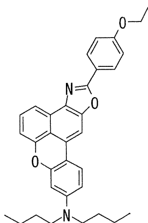
compound 14
