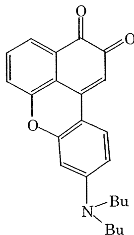
compound 7
