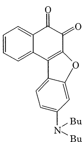
compound 6
