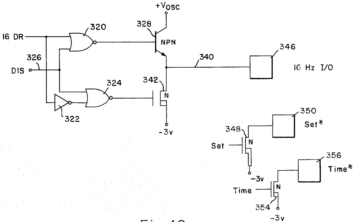
Fig. 10. OUTPUT BUFFERS CIRCUITS 102
