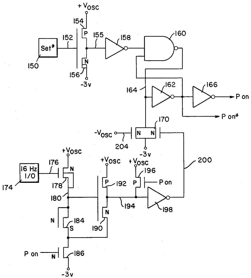
Fig. 7. POWER ON CIRCUIT 94
