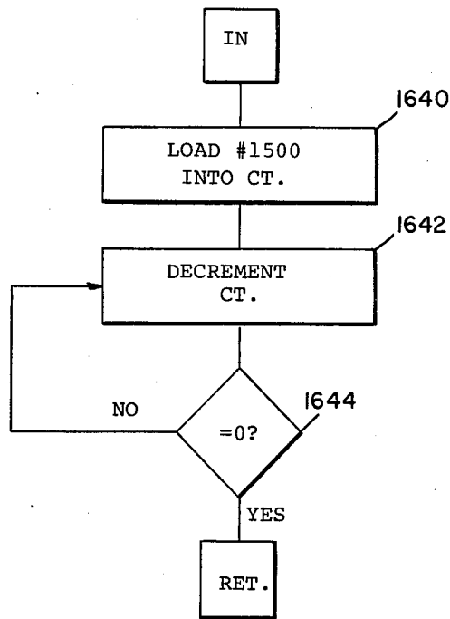
Fig. 54. DELAY SUBROUTINE 180 MILLISECONDS
