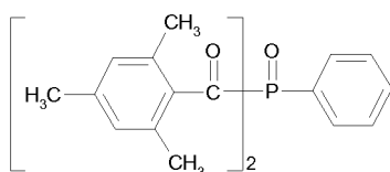
Bis(2,4,6-trimethylbenzoyl)- phenylphosphine oxide
