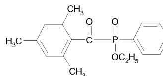
2,4,6-Trimethylbenzoyl-phenyl phosphinic acid ethyl ester
