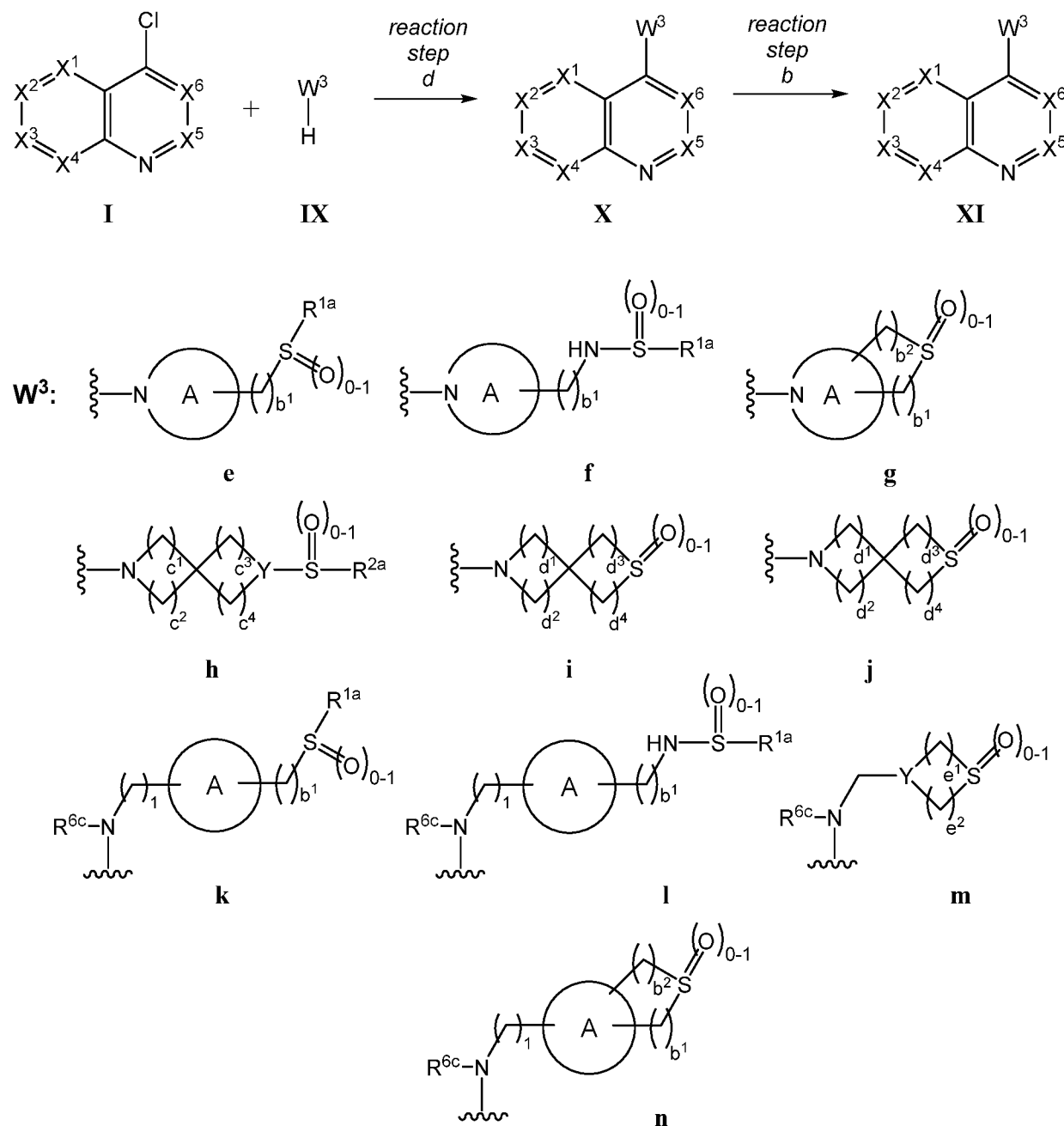
Scheme 3.
