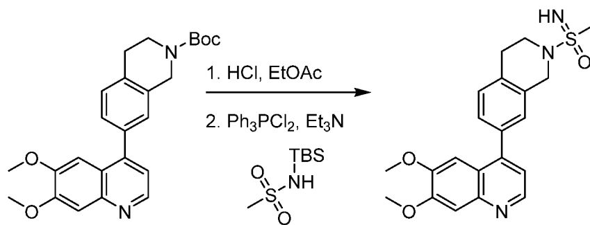
Compound 161
