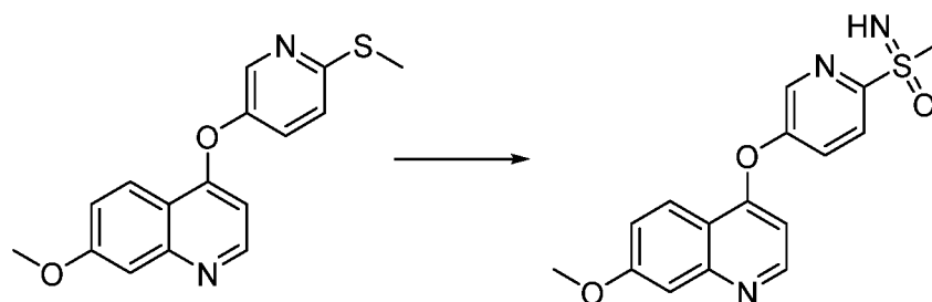
Compound 101
