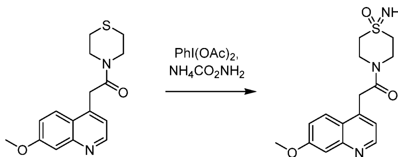
Compound 26
