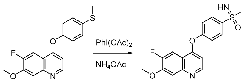
Compound 114
