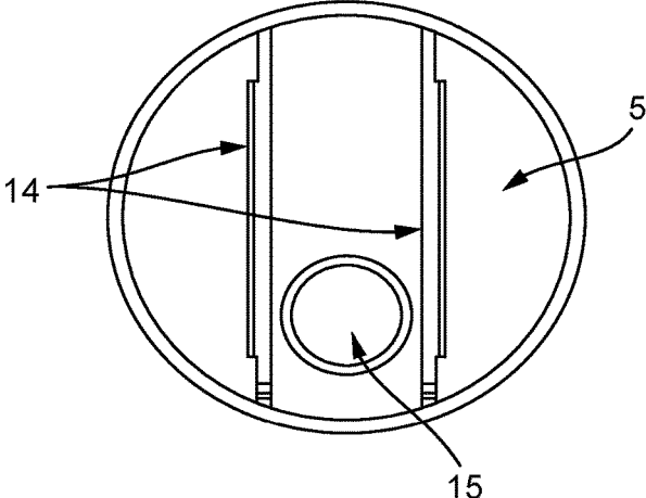
Figure 4: Bottom view of the disc shaped closure
