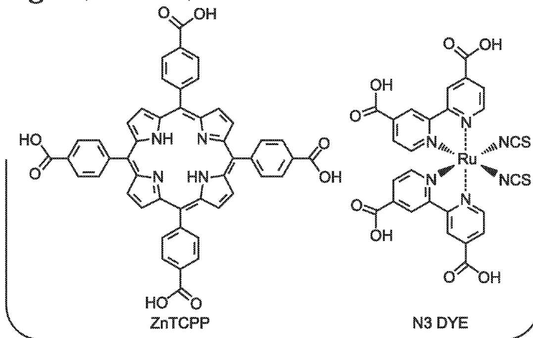
Fig. 5 (PRIOR ART)
