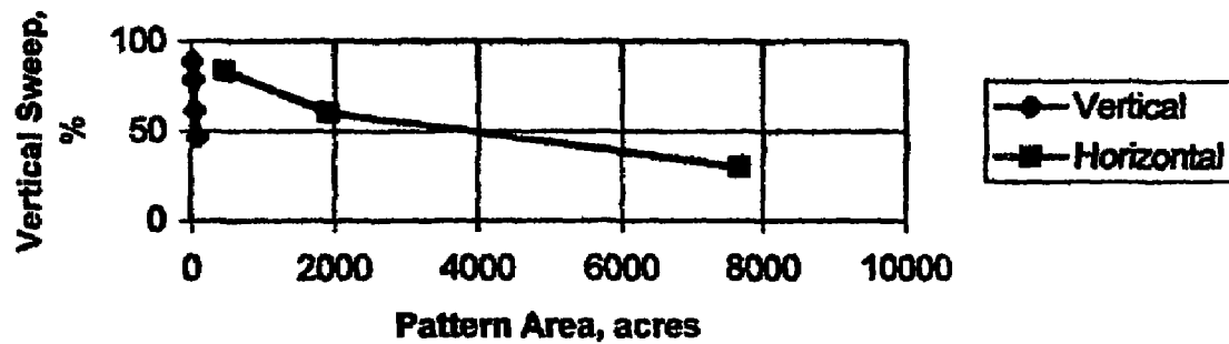
FIG. 16. SWEEP VERSUS PATTERN AREA, MAXIMUM INJECTION RATE
