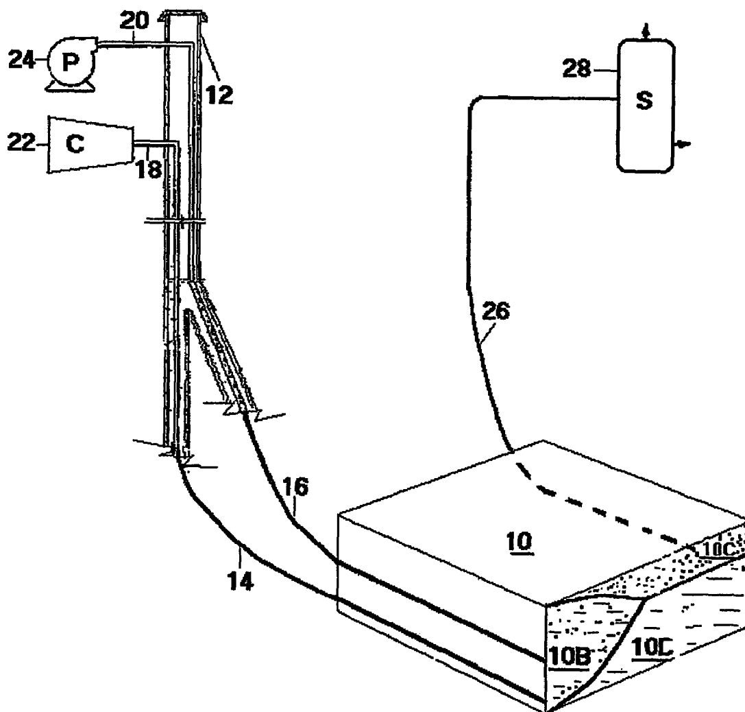
FIG. 1. HORIZONTAL WELL APPLICATION IN A PATTERN ELEMENT
