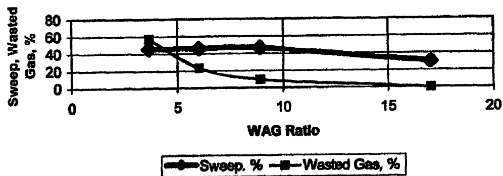
FIG. 10. WAG RATIO SELECTION
