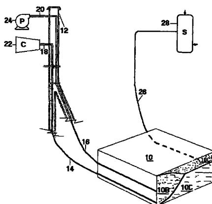
HORIZONTAL WELL APPLICATION IN A PATTERN ELEMENT
