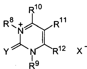
(Ca-II)
