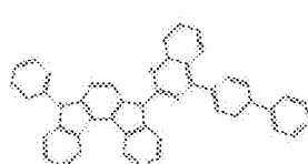
Compound 8
