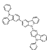
Compound 3
