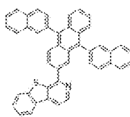
Compound 6
