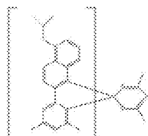
Compound 10
