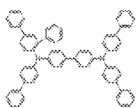
Compound 2
