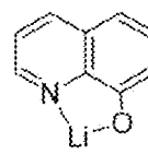
Compound 7
