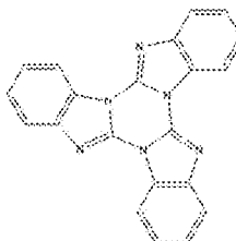
Compound 15
