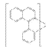
Compound 9
