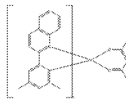
Compound 12
