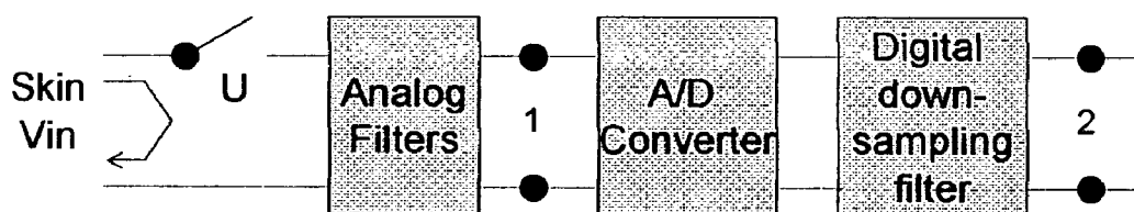
b) Front-end circuitry of DEVICE_B
