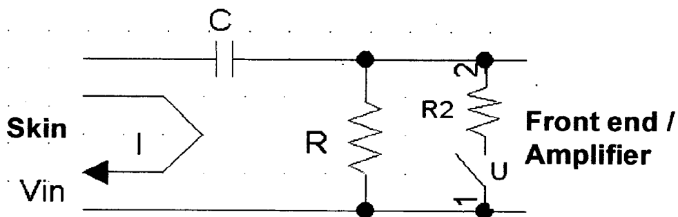
b) Front-end circuitry of Device A
