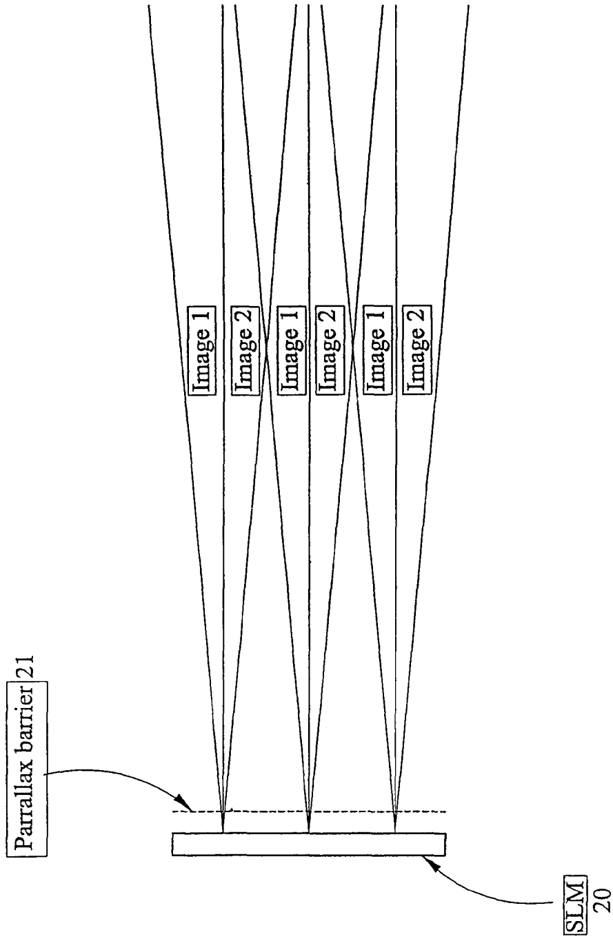
FIG 2 Conventional Art
