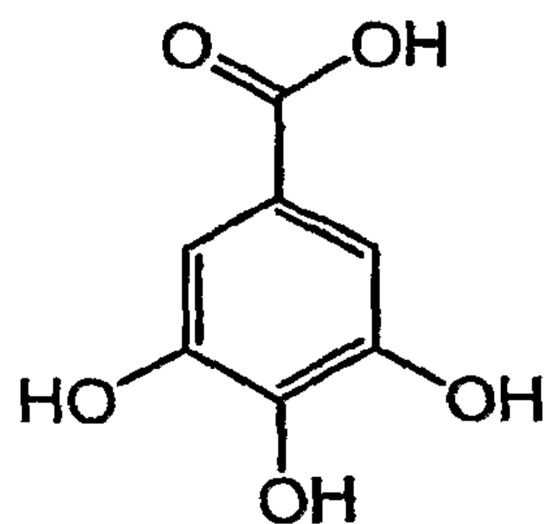
Gallic acid
