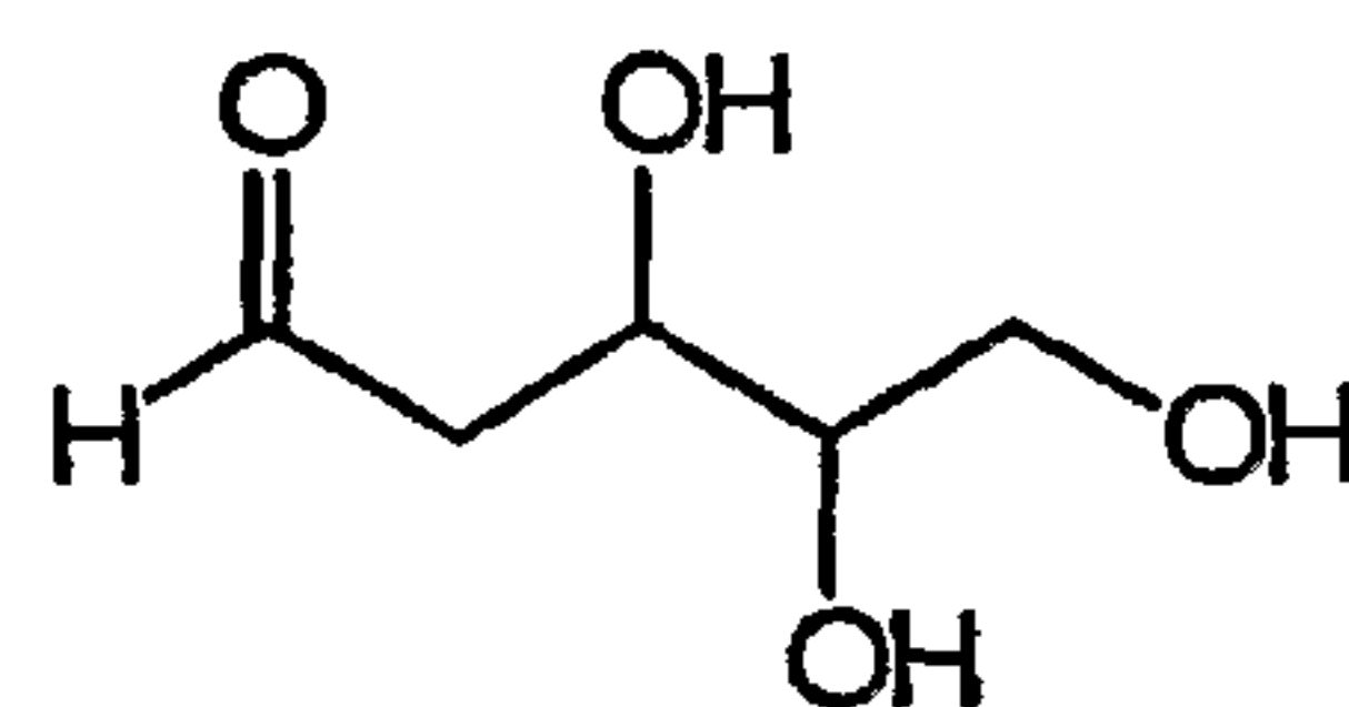
2-Deoxy-D-ribose
