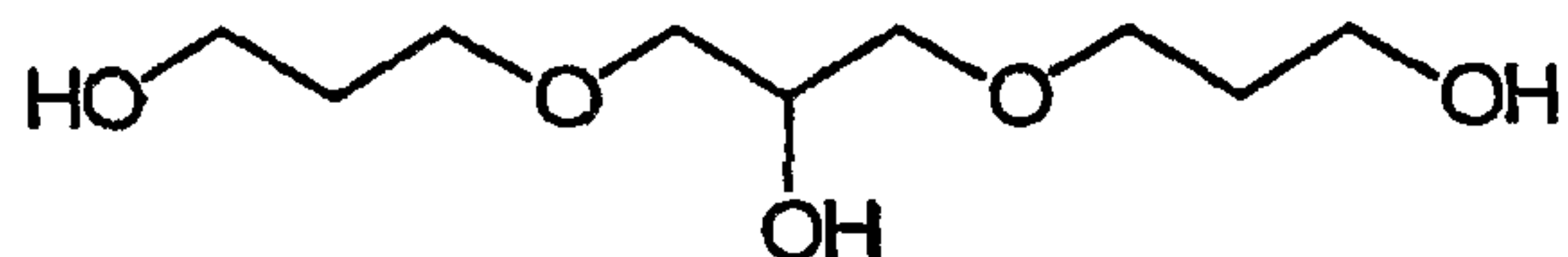
1,3-Di(hydroxypropoxy)-2-hydroxyl-propane
