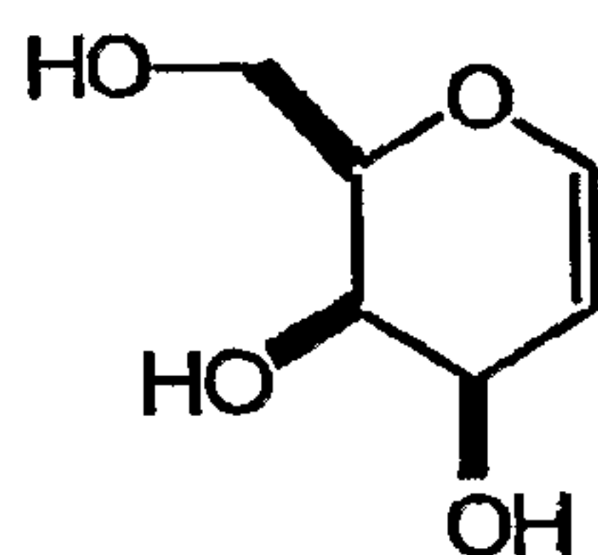
D-Galactool
