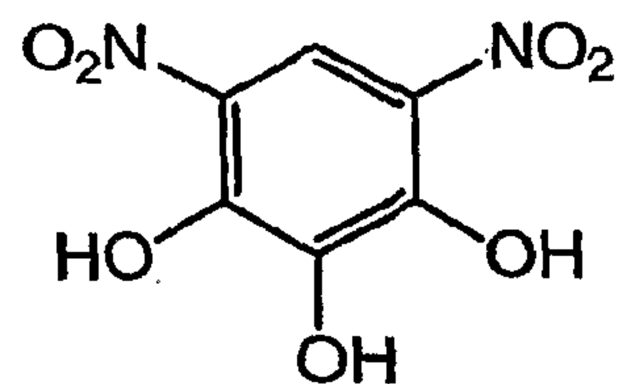
4,6-Nitropyrogallol
