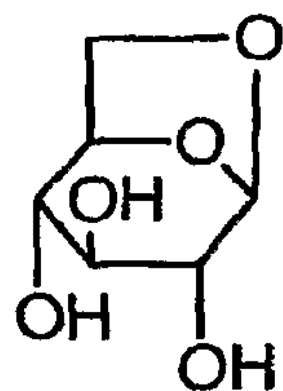
1,6-anhydro- \beta -D-Glucose
