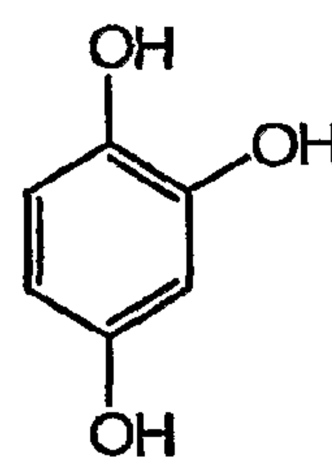
1,2,4,-Trihydroxyl-benzene
