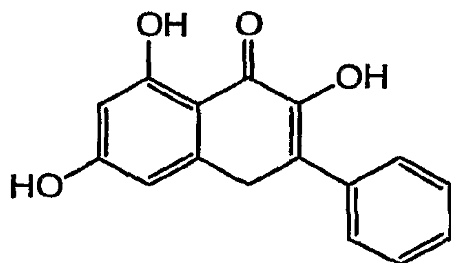
3,5,7-Trihydroxyflavone
