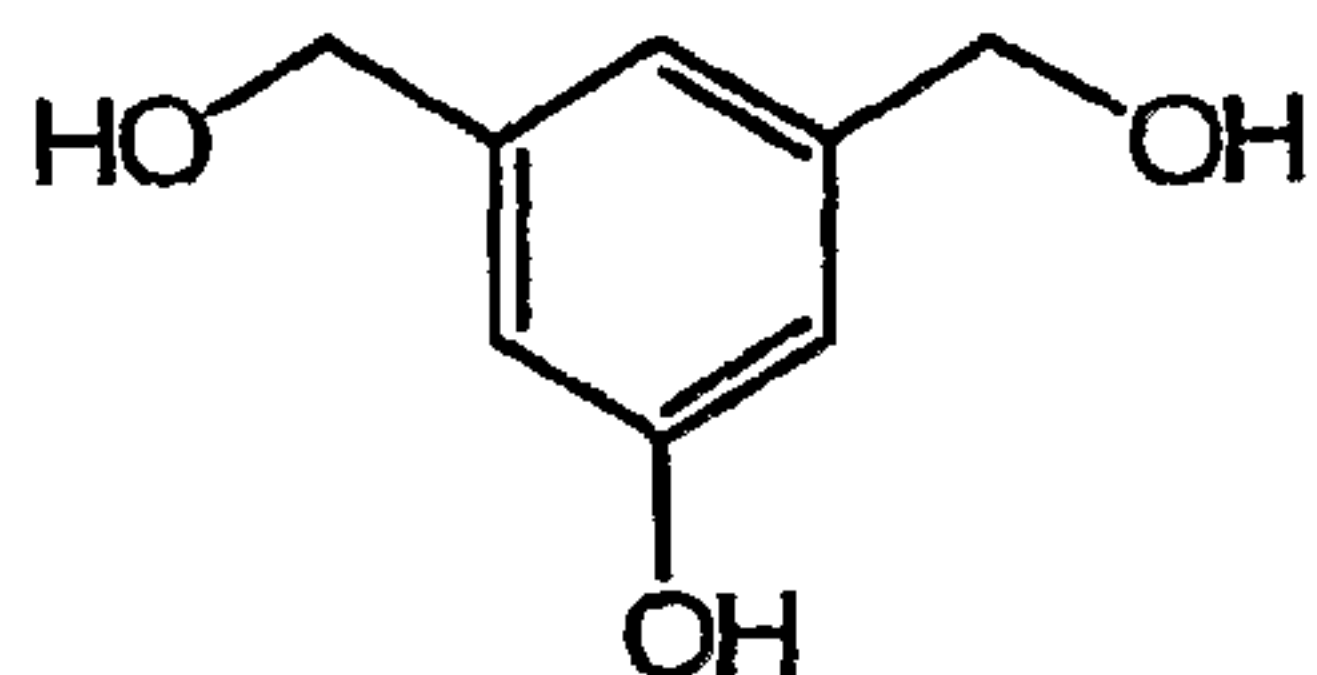
3,5,-Di(hydroxymethyl)phenol
