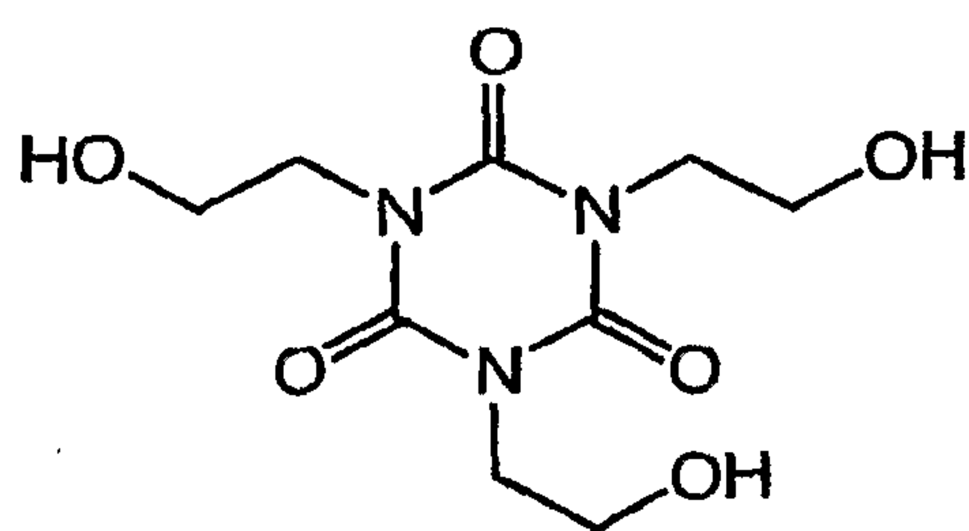
1,3,5-Tris(2-hydroxyethyl)-Cyanuric acid
