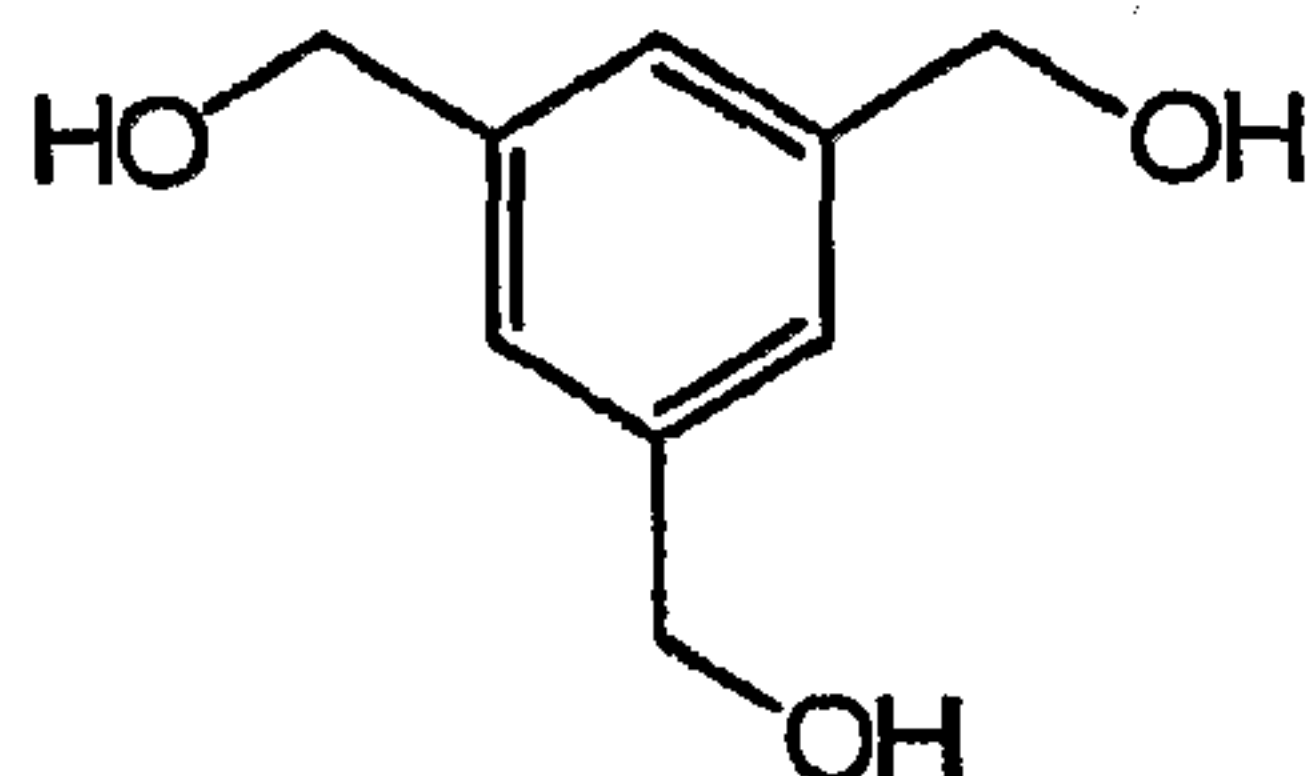
1,3,5,-Tri(hydroxymethyl)benzene
