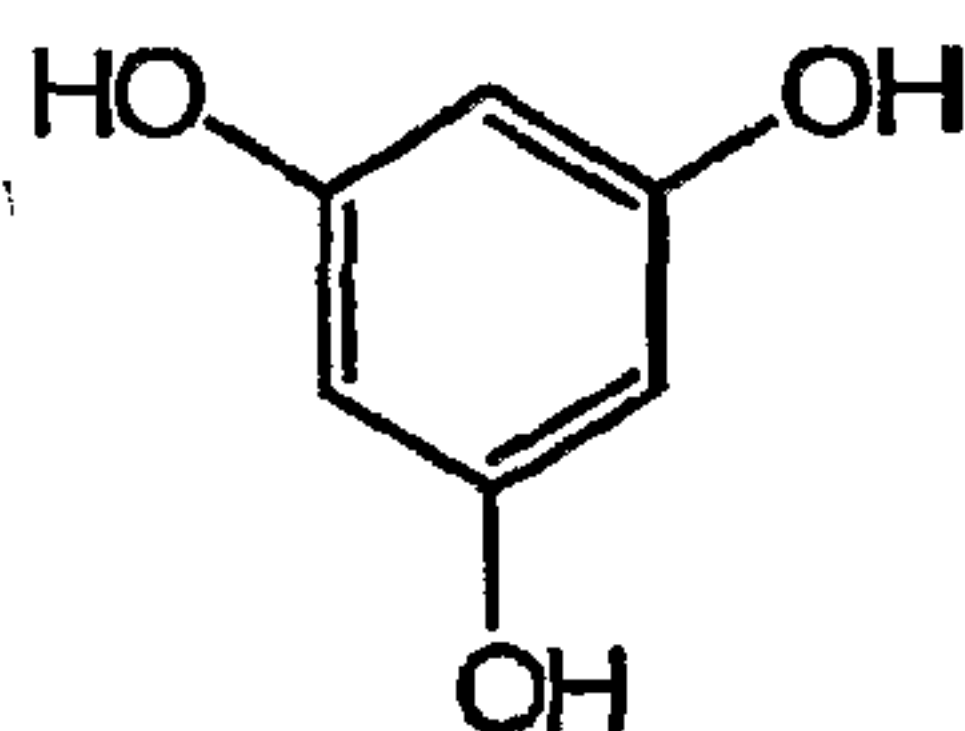
1,3,5,-Trihydroxyl-benzene
