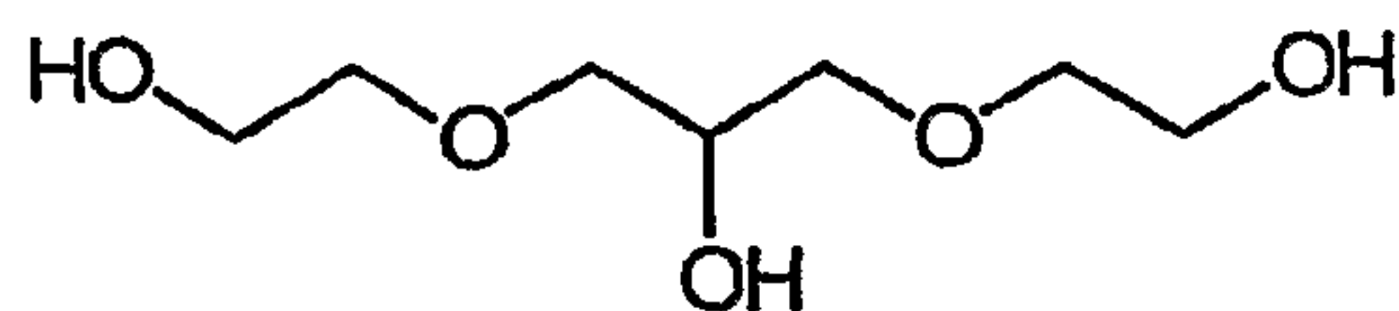
1,3-Di(hydroxyethoxy)-2-hydroxyl-propane
