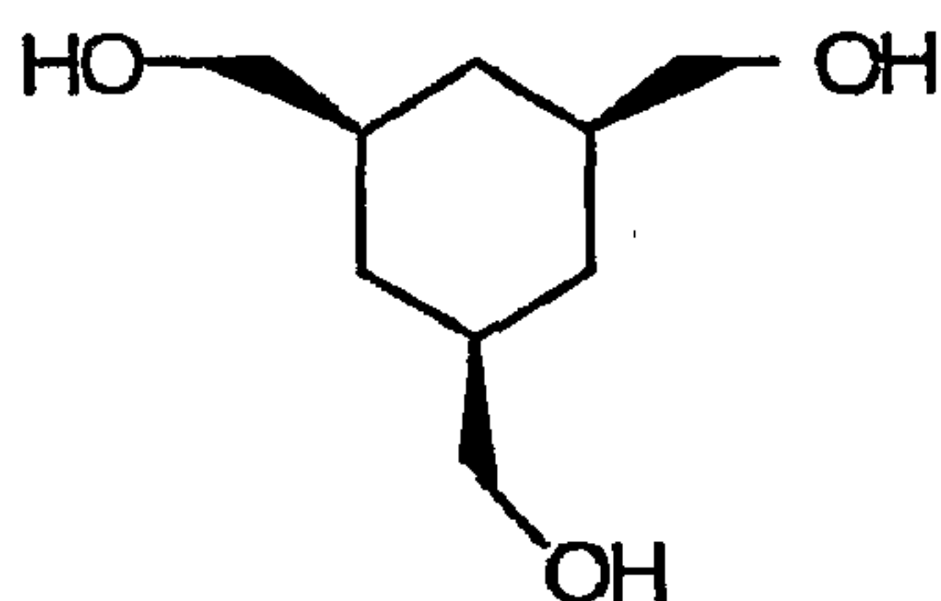
cis-1,3,5-Tri(hydroxymethyl)cyclohexane
