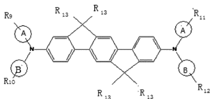
structural formula (3)
