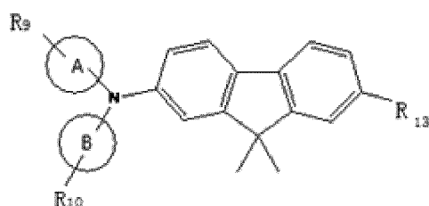
structural formula (6)
