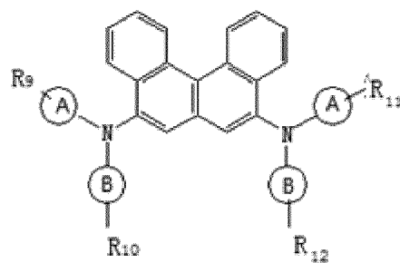
structural formula (4)
