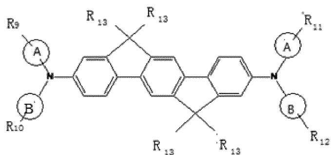
structural formula (3)
