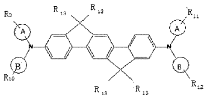
structural formula (3)
