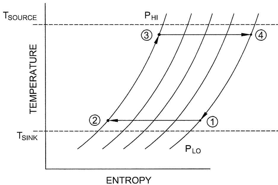
Fig. 3 (Prior Art)
