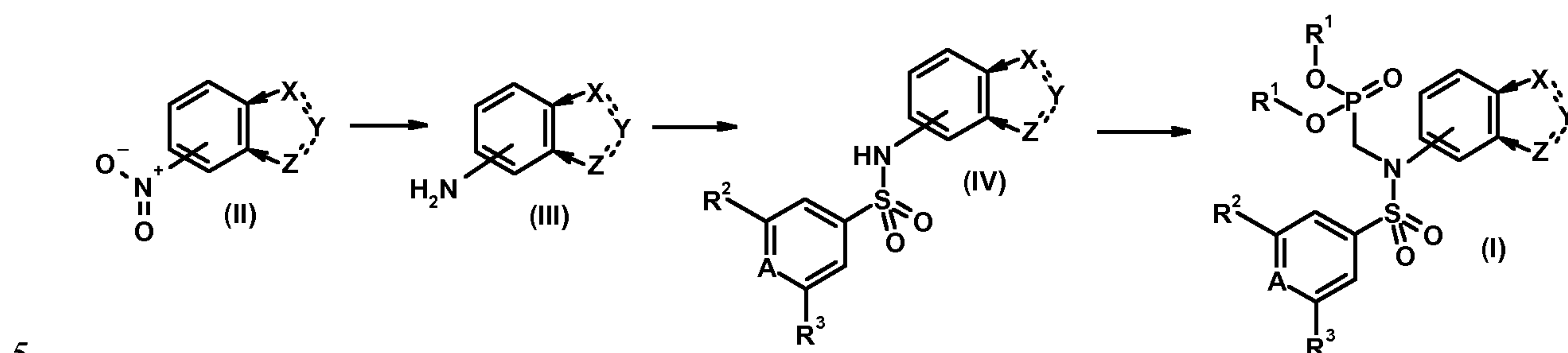
Scheme 1
