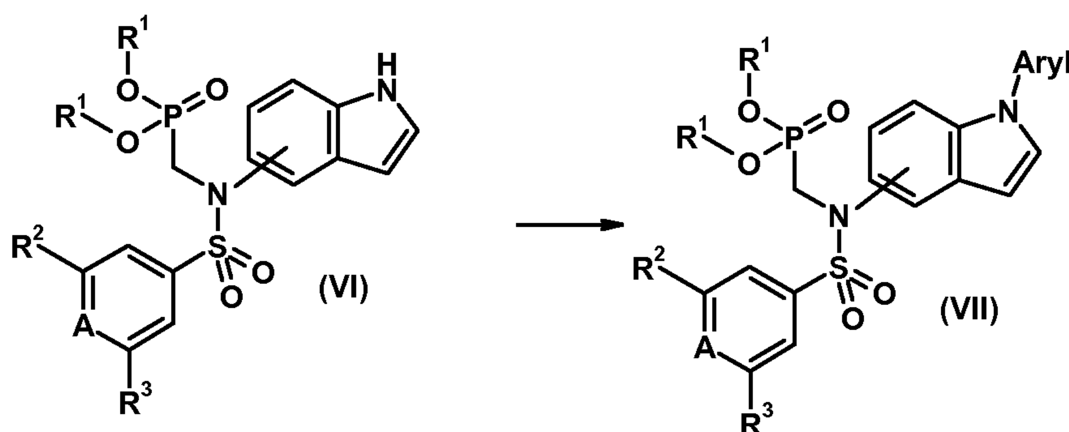
20 Scheme 3
