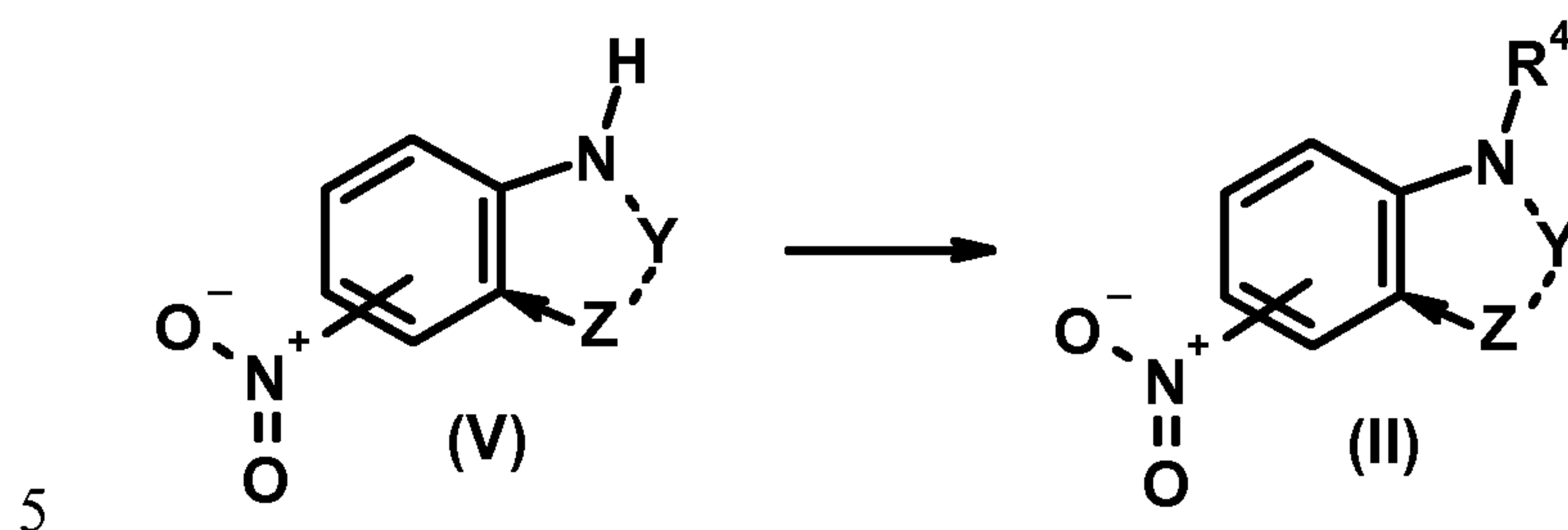
Scheme 2
