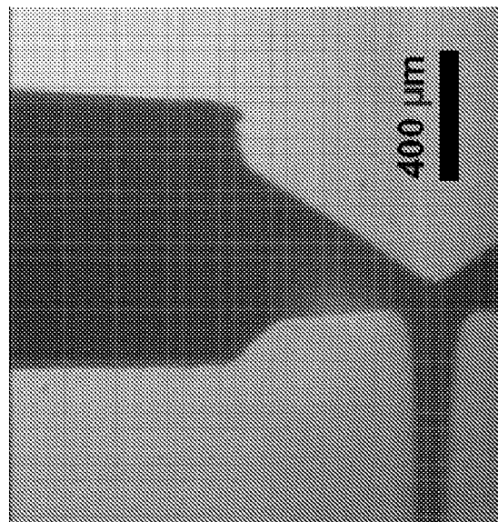
Taylor cone contact mode direct writing \text{TiO}_2 NP paste
