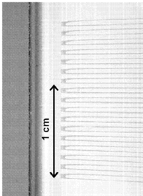
Single pass \text{TiO}_2 NP pattern on FTO (500 \mu\text{m} pitch, 100 \mu\text{m} line width)
