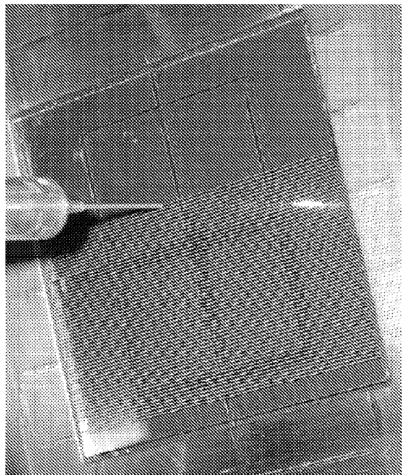
100um Fodel silver paste lines patterned on uncoated insulating glass (5cm x 5cm)
