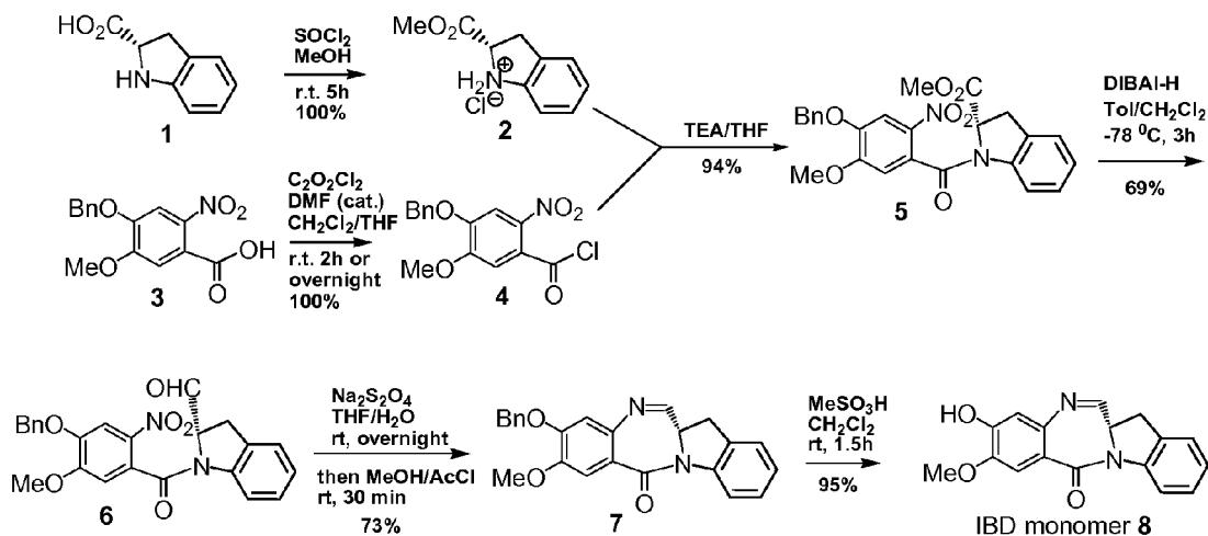
FIG. 1 Synthetic scheme of IBD monomer 8
