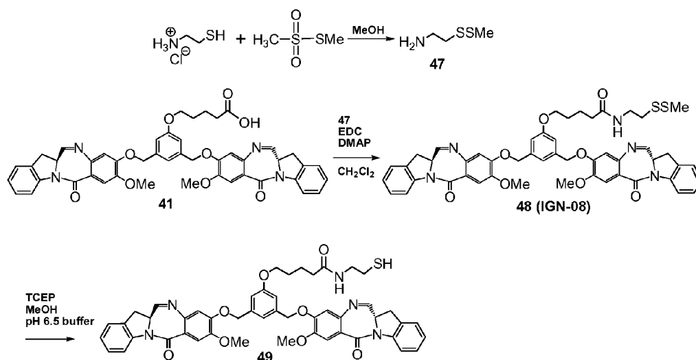
FIG. 9 Synthetic scheme of thiol 49
