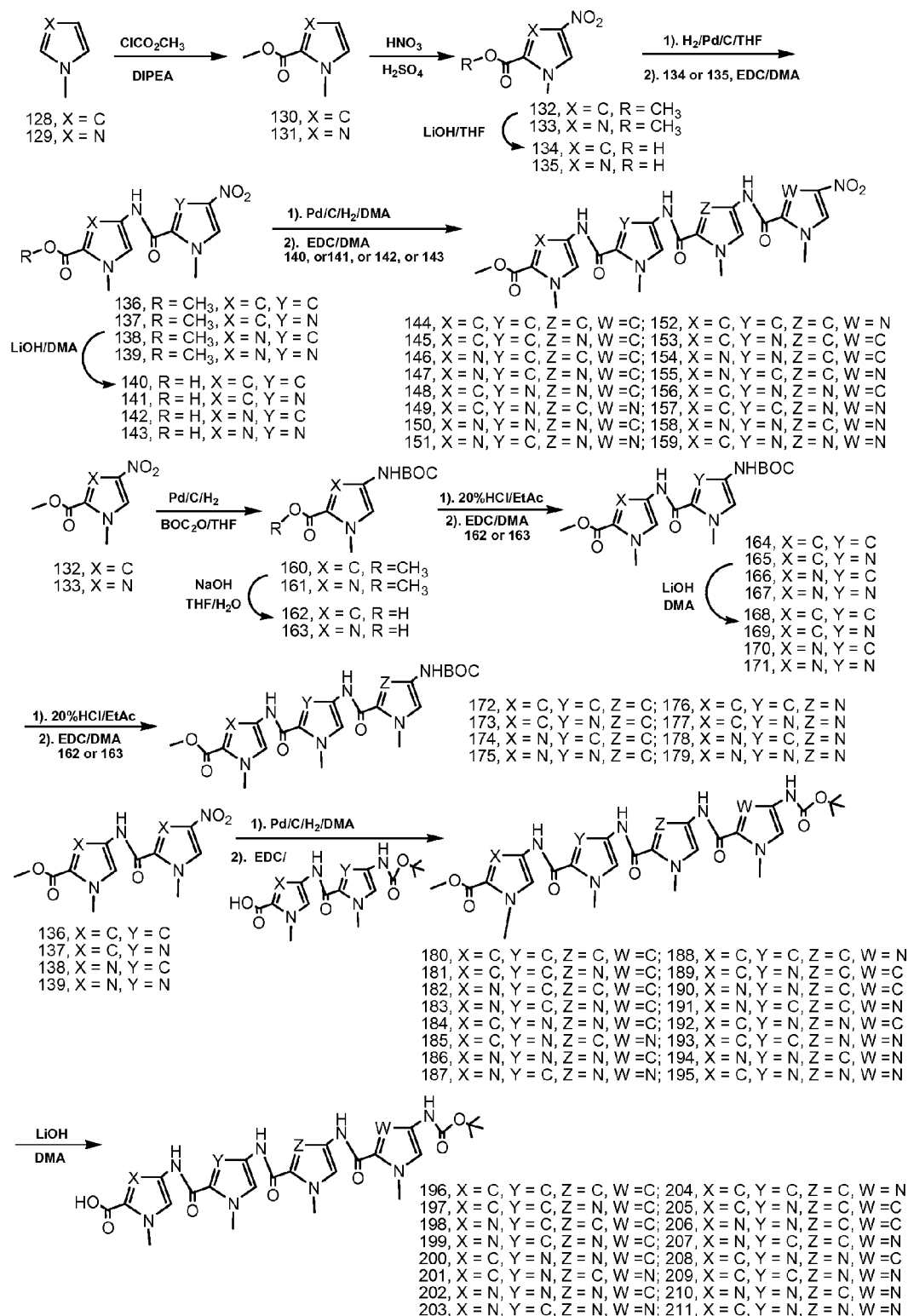
FIG. 18 The assembling of polypyrroles/polyimidazoles
