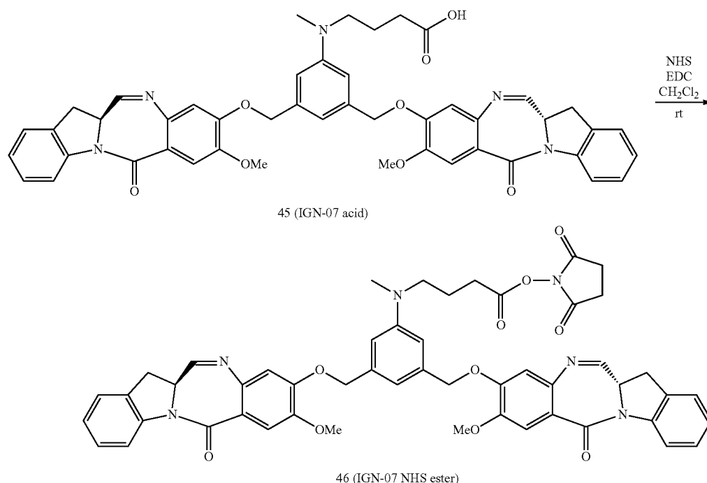
Compound 46
