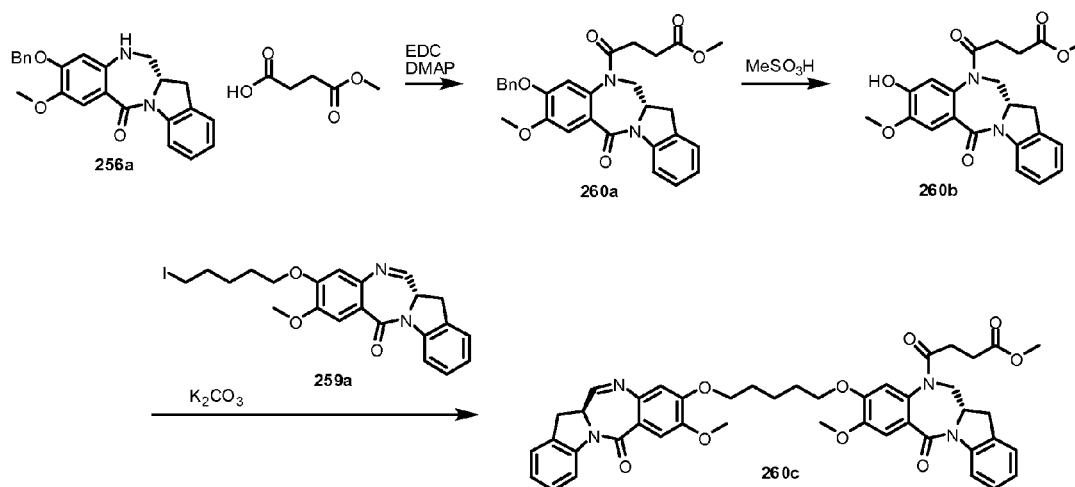
FIG. 43 Synthetic scheme of compound 260c (IGN-25-OMe).
