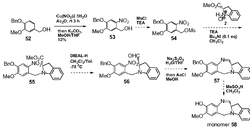
FIG. 12 Synthetic scheme of isoindolinobenzodiazepine monomer 66
