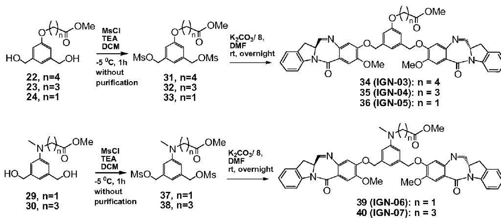
FIG. 7 Synthetic scheme of dimers 34 , 35 , 36 , 39 and 40 (IGN-03~07)
