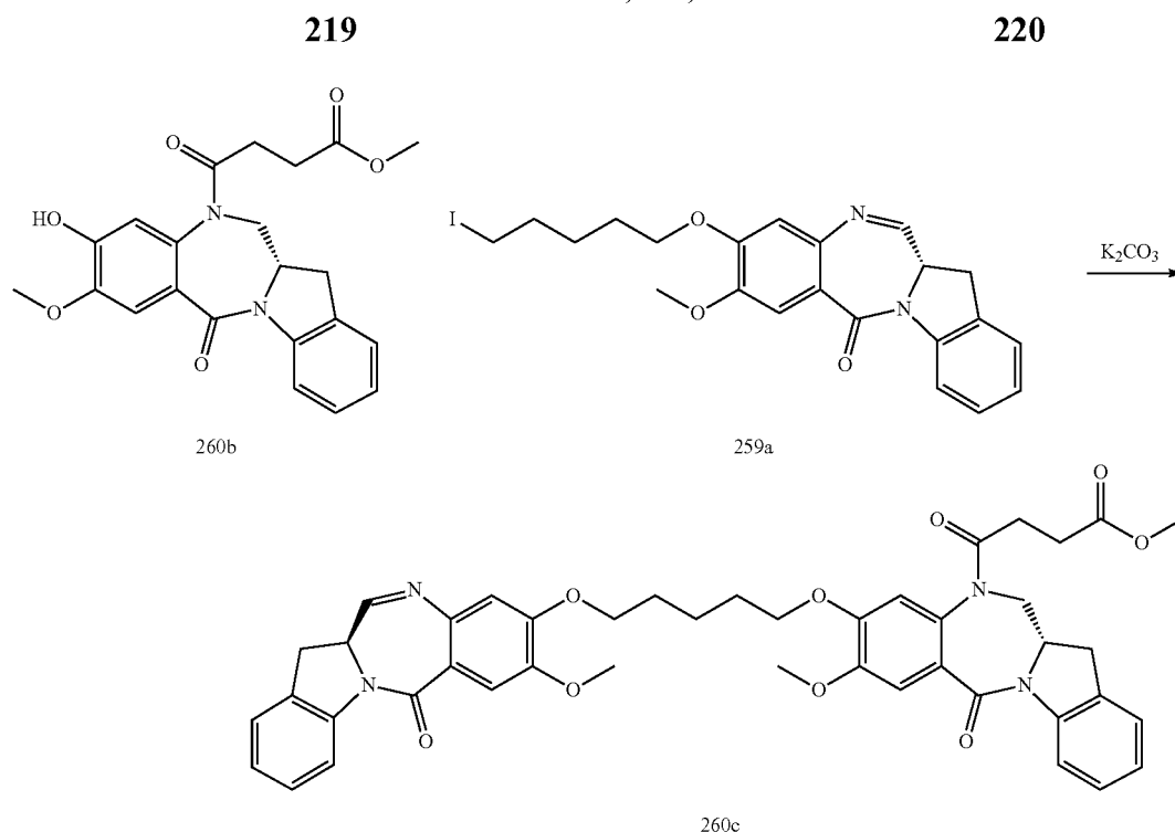
Compound 260c
