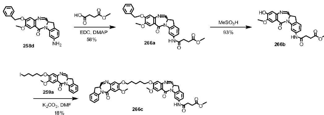
FIG. 48 Synthetic scheme of dimer 266c (IGN-22-OMe).
