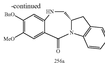
Compound 256a
