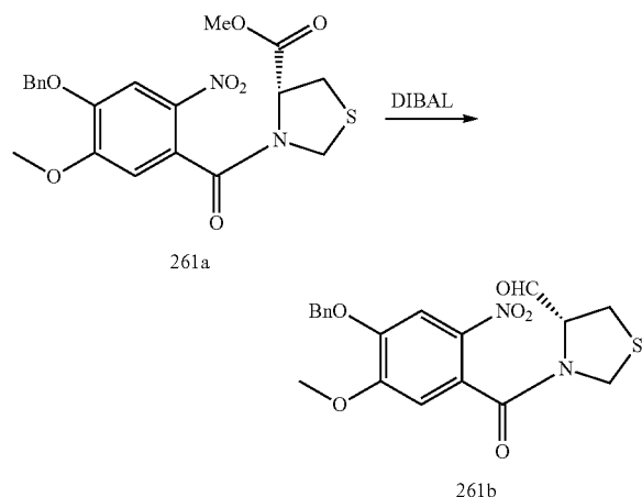
Compound 261b
