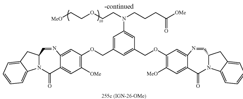
Compound 255c (IGN-26-OMe)
