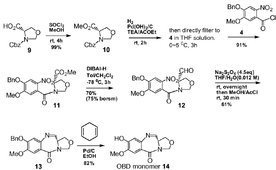
FIG. 2 Synthetic scheme of OBD monomer 14
