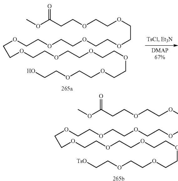
methyl 1-(tosyloxy)-3,6,9,12,15,18,21,24,27,30,33,36-dodecaoxanonatriacontan-39-oate (265b)
