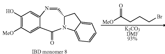
IBD monomer 8
