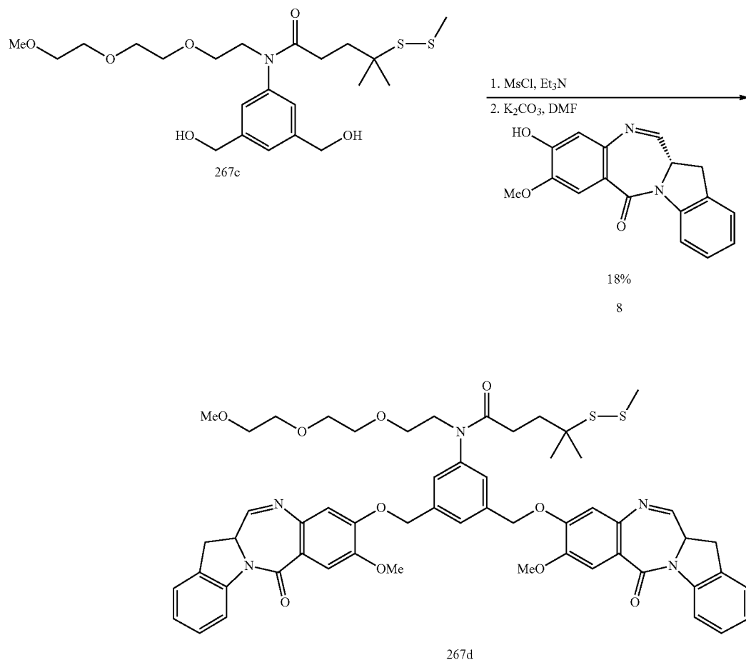
Compound 267d
