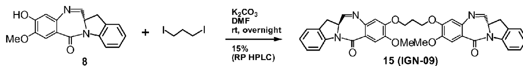
FIG. 3 Synthetic scheme of dimer 15 (IGN-09)
