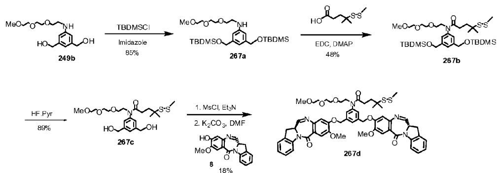
FIG. 49 Synthetic scheme of dimer 267d (IGN-31-SMe).
