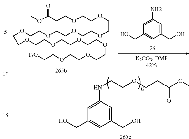
methyl 1-(3,5-bis(hydroxymethyl)phenylamino)-3,6,9,12,15,18,21,24,27,30,33,36-dodecaoxanonatriacontan-39-oate (265c)
