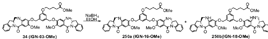
FIG. 34 Synthetic scheme of esters of IBD dimers
