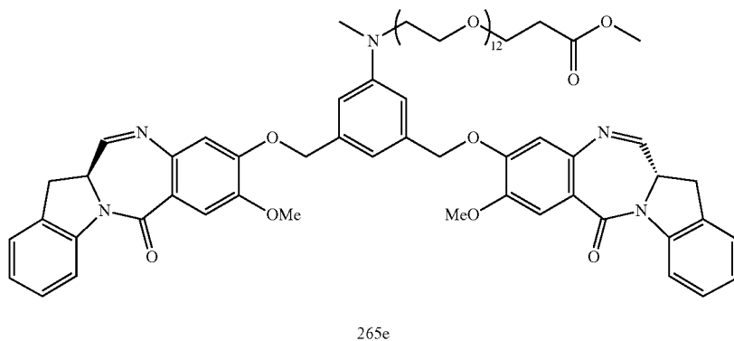
Compound 265e
