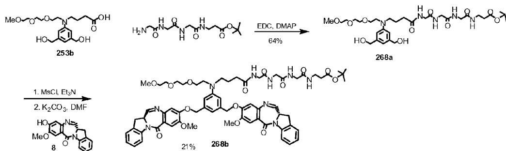
FIG. 50 Synthetic scheme of dimer 268b (IGN-32-OtBu).
