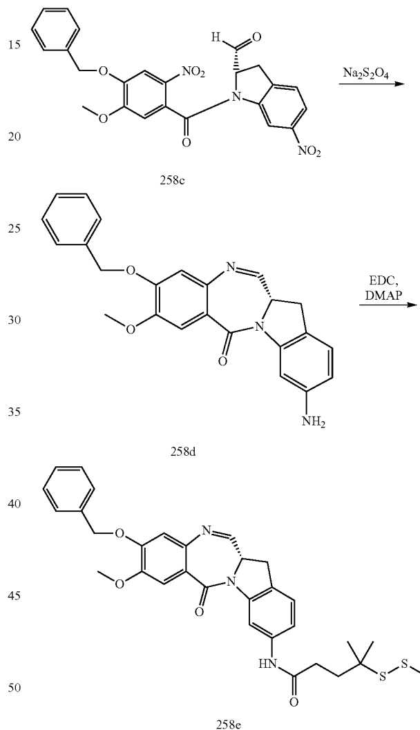
Compound 258e
