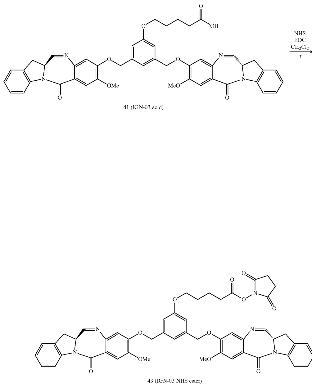
Compound 43
