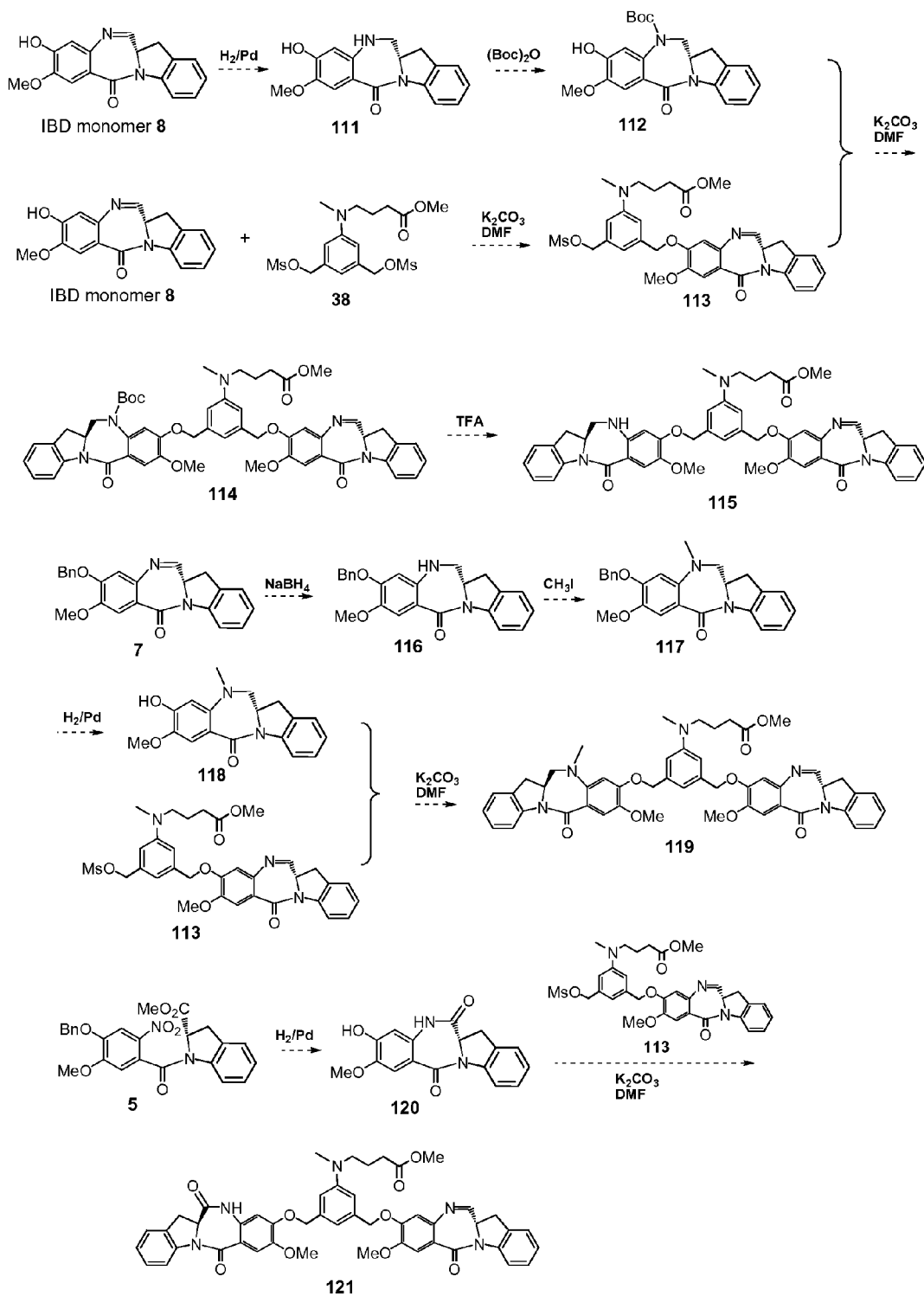
FIG. 16 Synthetic schemes of compounds 115, 119 and 121
