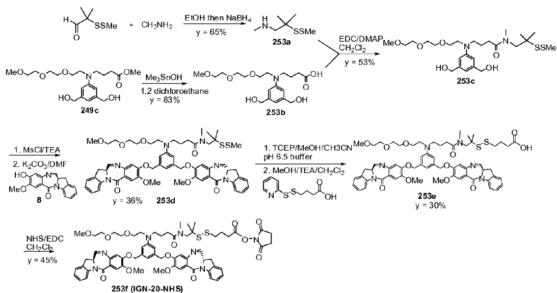
FIG. 37 Synthetic scheme for linkable dimer
