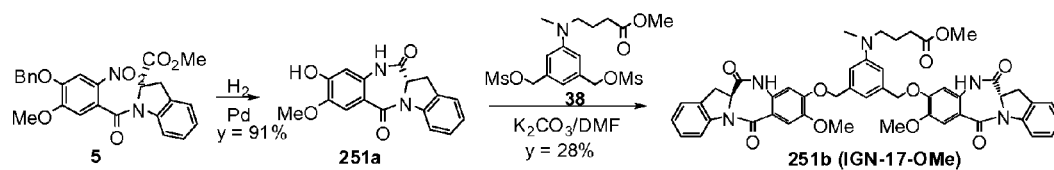
FIG. 35 Synthetic scheme of dimer 251b (IGN-17-OMe).
