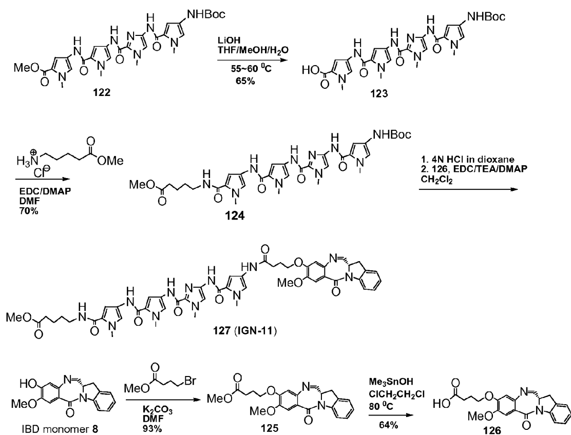
FIG. 17 Synthetic scheme of compound 127 (IGN-11)
