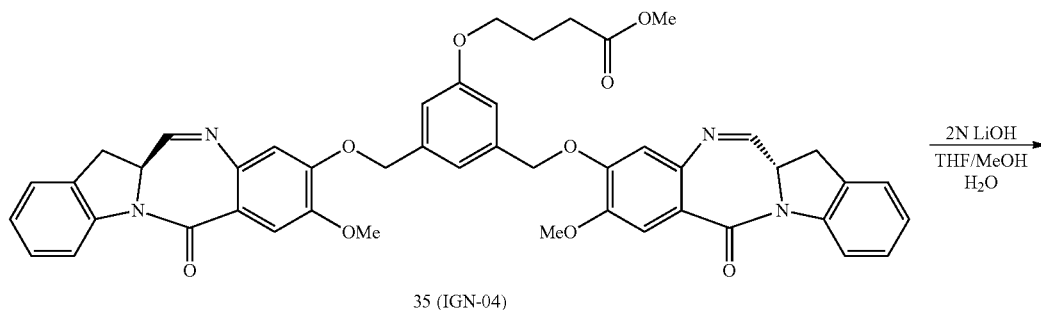
Compound 42
