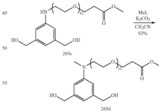
methyl 2-(3,5-bis(hydroxymethyl)phenyl)-5,8,11,14,17,20,23,26,29,32,35,38-dodecaoxa-2-azahentetracontan-41-oate (265d)
