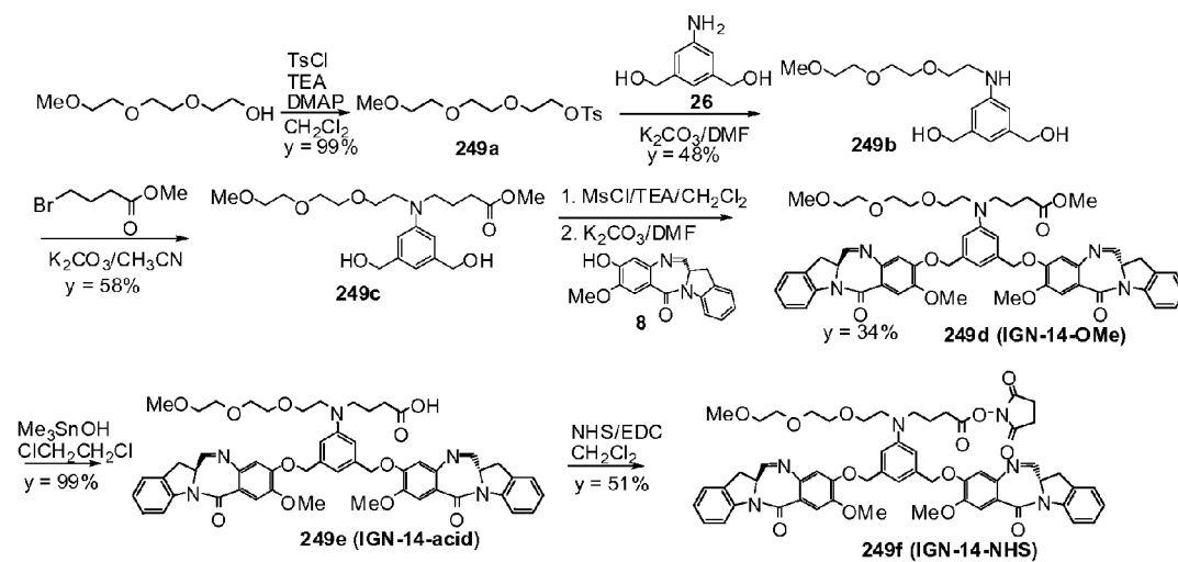
FIG. 33 Synthetic scheme for indolinobenzodiazepine (IBD) dimers
