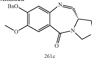
Compound 261c
