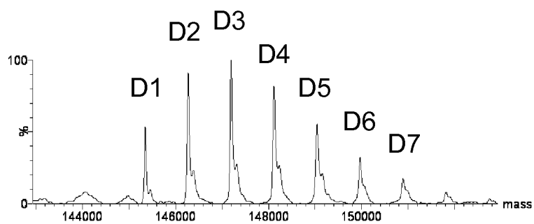
FIG. 59 MS analysis of chB38.1-IGN14 conjugate
