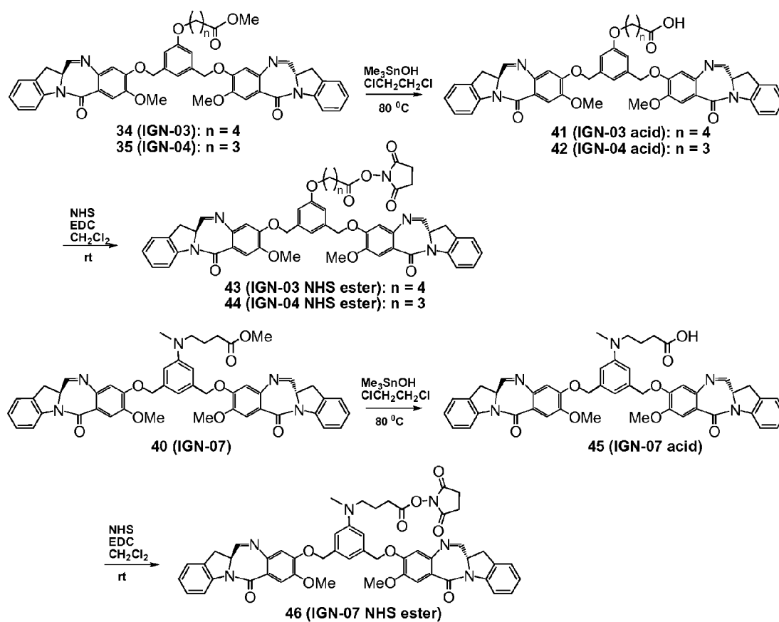
FIG. 8 Synthetic scheme of the NHS esters 43 , 44 and 46
