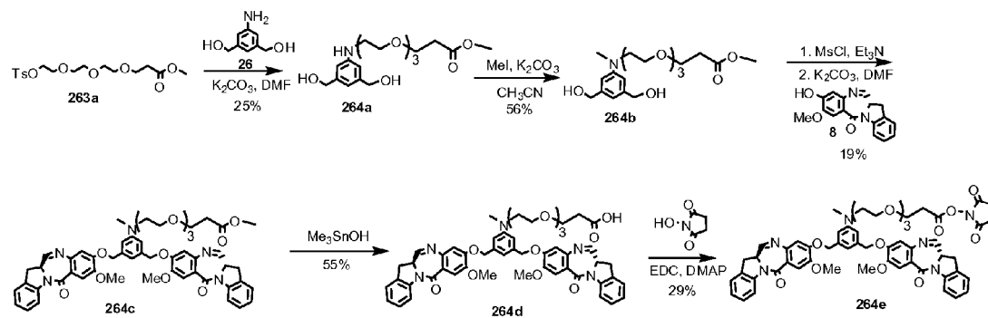
FIG. 46 Synthetic scheme of dimer 264e (IGN-27-NHS).
