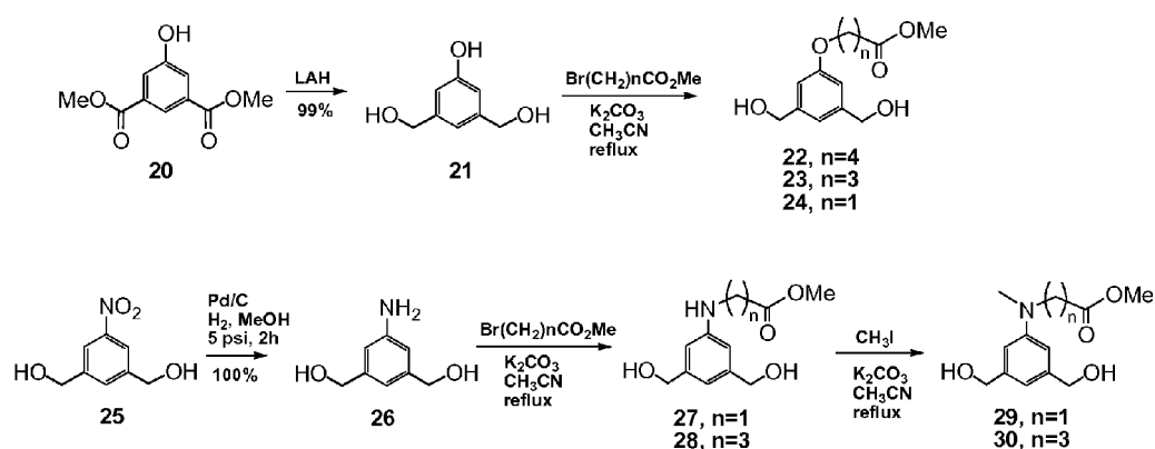
FIG. 6 Synthetic scheme of the linkers
