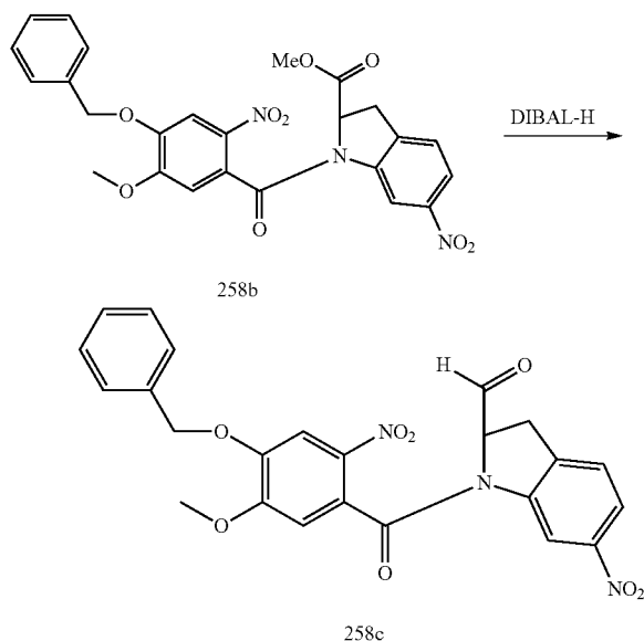
1-(4-(benzyloxy)-5-methoxy-2-nitrobenzoyl)-6-nitroindoline-2-carbaldehyde (258c)
