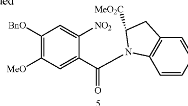
(2S)-1-[5-methoxy-2-nitro-4-(phenylmethoxy)-benzoyl]-2-indolinealdehyde 6
