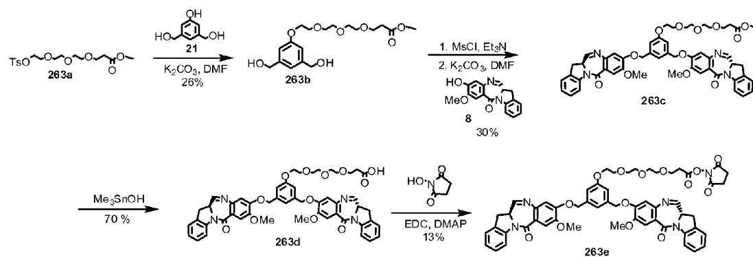
FIG. 45 Synthetic scheme of dimer 263e (IGN-13-NHS).
