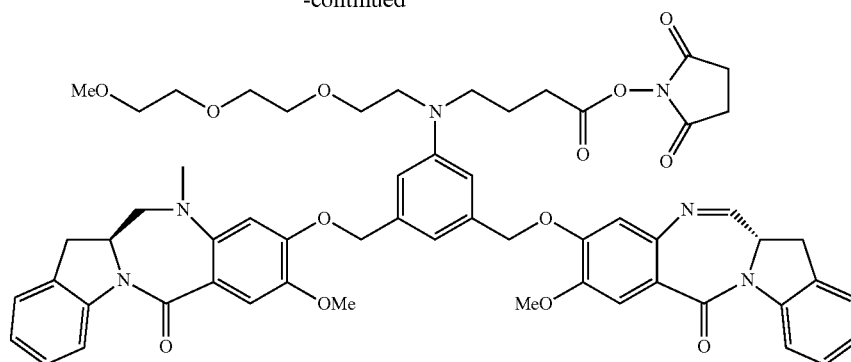
256g (IGN-29-NHS)
