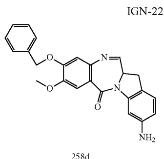
258d
