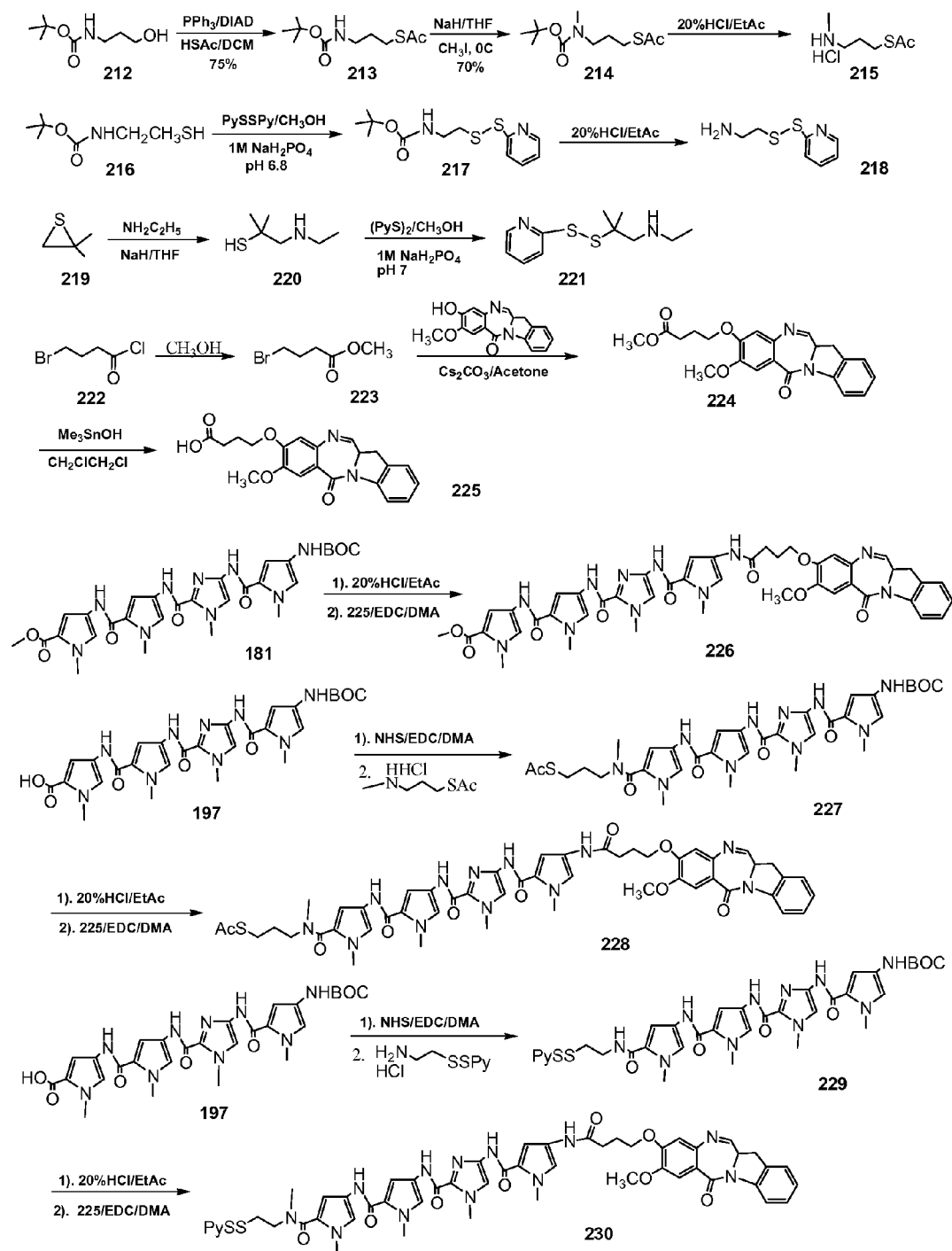
FIG. 19 The synthesis of IBD-polypyrrole-imidazole analogs
