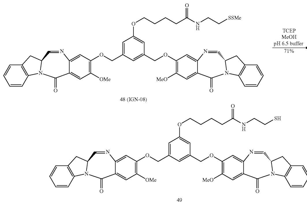
Compound 49
