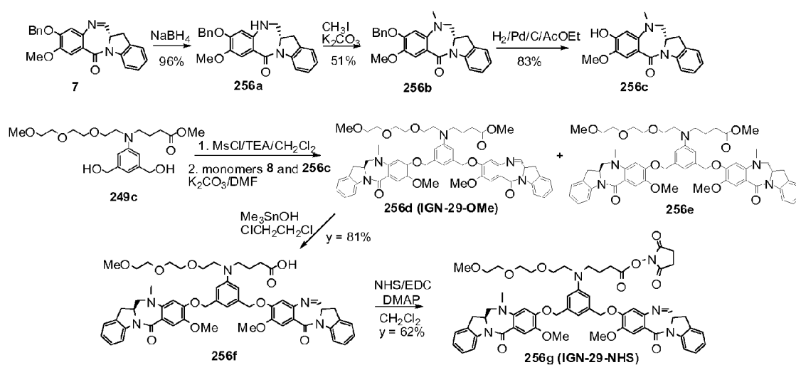
FIG. 40 Synthetic scheme of compound 256g (IGN-29-NHS).
