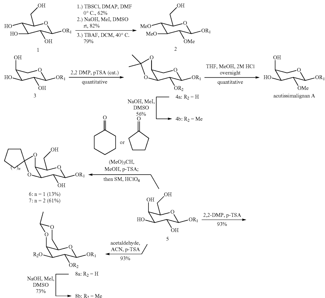
Scheme 1: Synthetic schemes for phyllanthusmin compounds.
