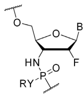
(IIIa)
