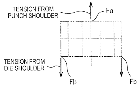
BEFORE MOLDING
