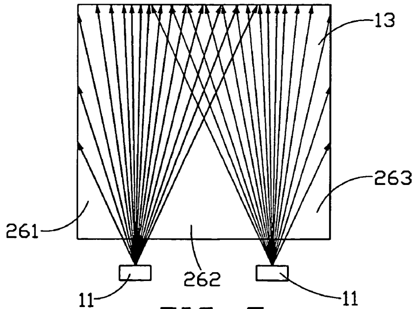
FIG. 5 (PRIOR ART)
