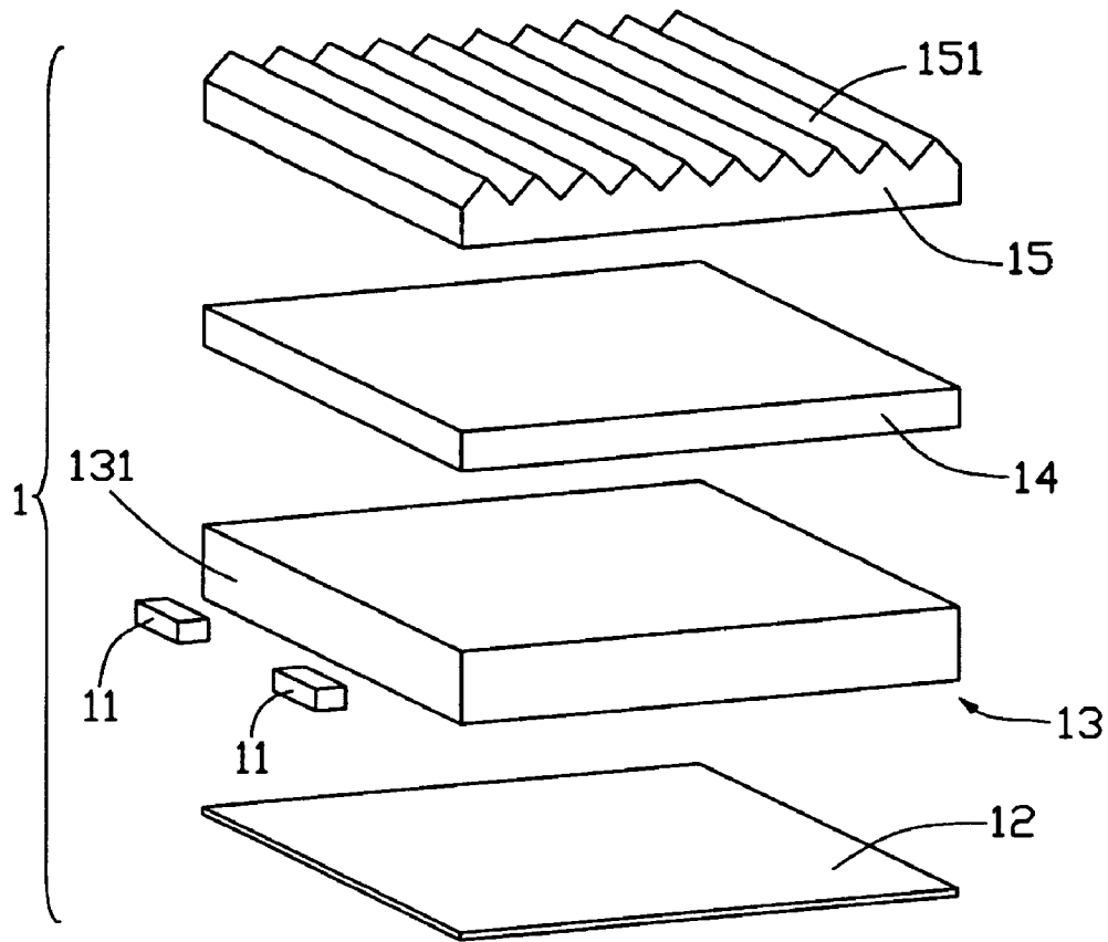
FIG. 4 (PRIOR ART)
