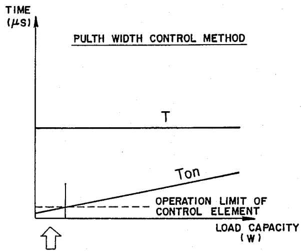
FIG. 13 (PRIOR ART)
