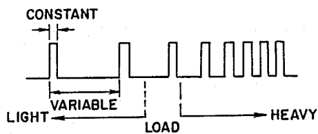
FIG. 8 (PRIOR ART)
