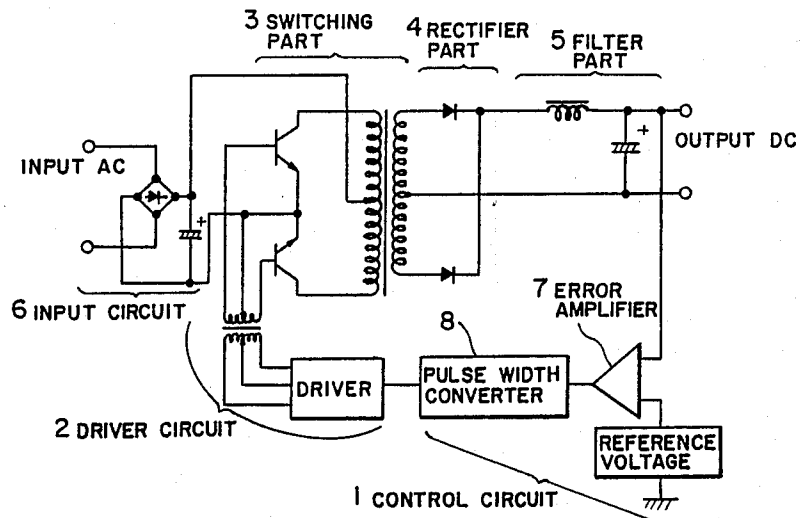
FIG. 9 (PRIOR ART)
