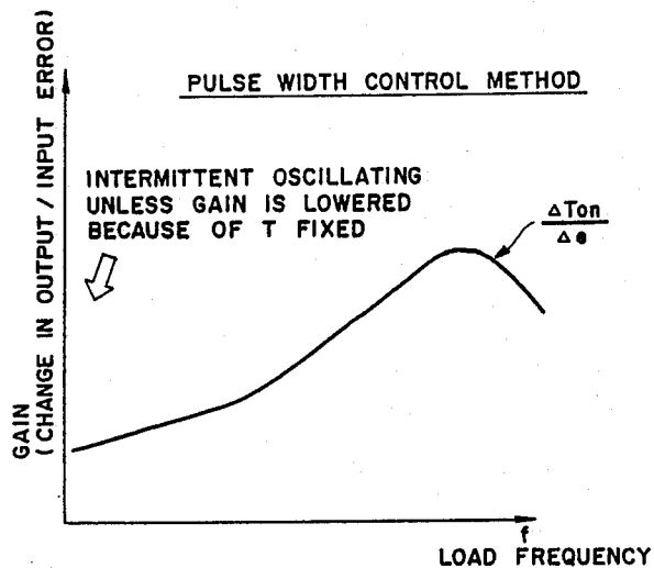
FIG.14 (PRIOR ART)
