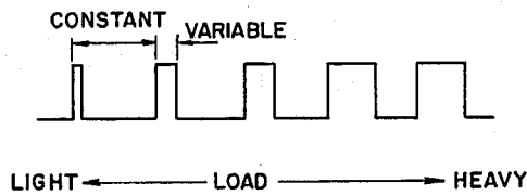
FIG. 11 (PRIOR ART)
