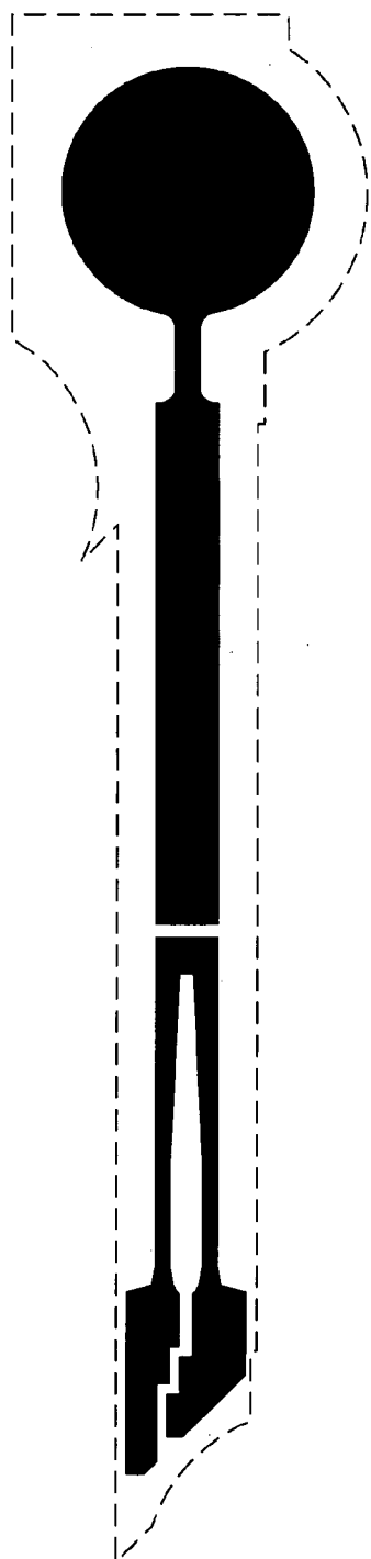
Heater mask
