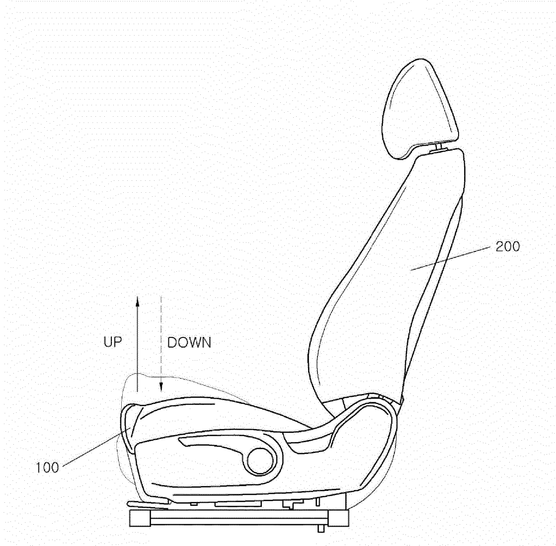
FIG.16 (RELATED ART)
