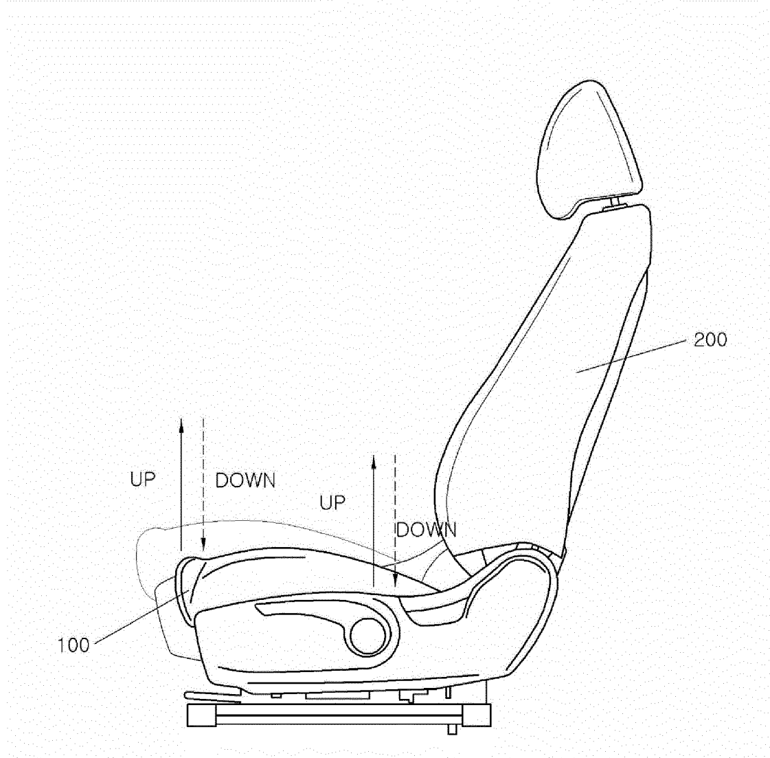
FIG.14 (RELATED ART)
