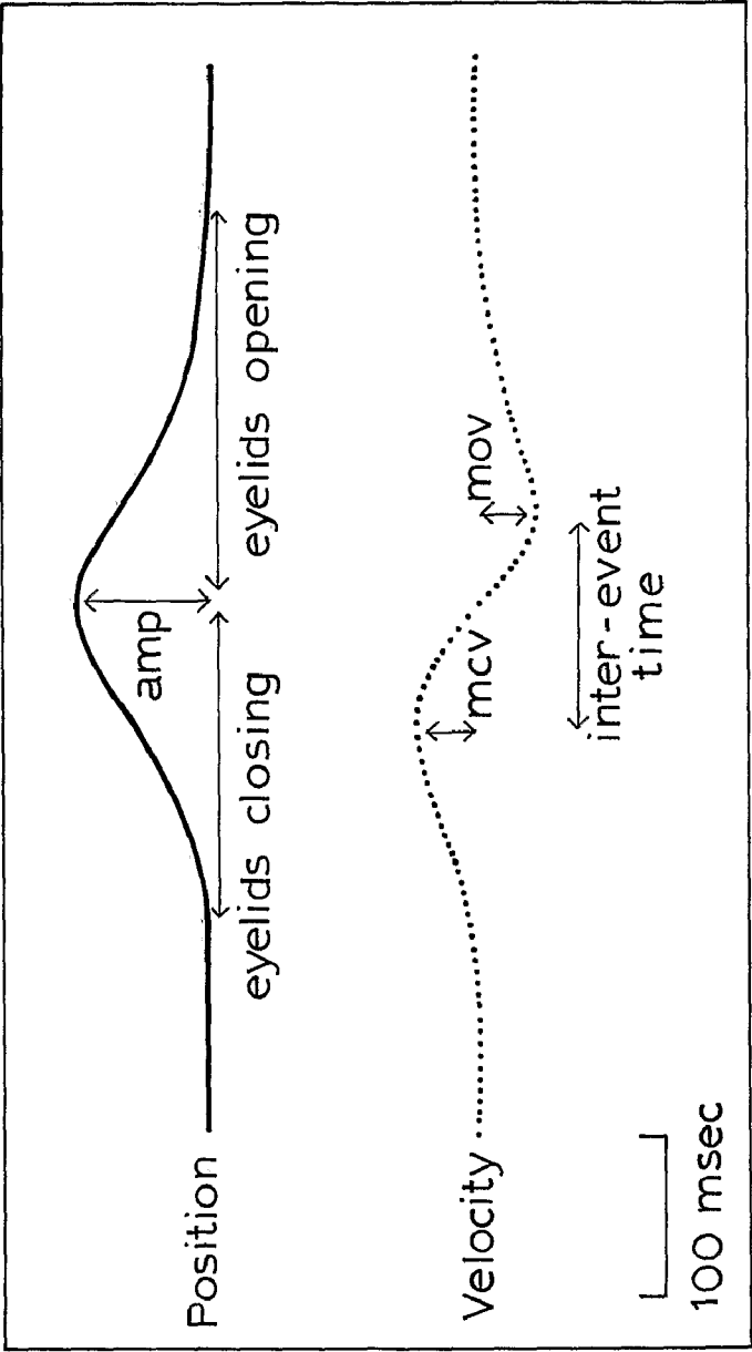
Blink in a drowsy subject
