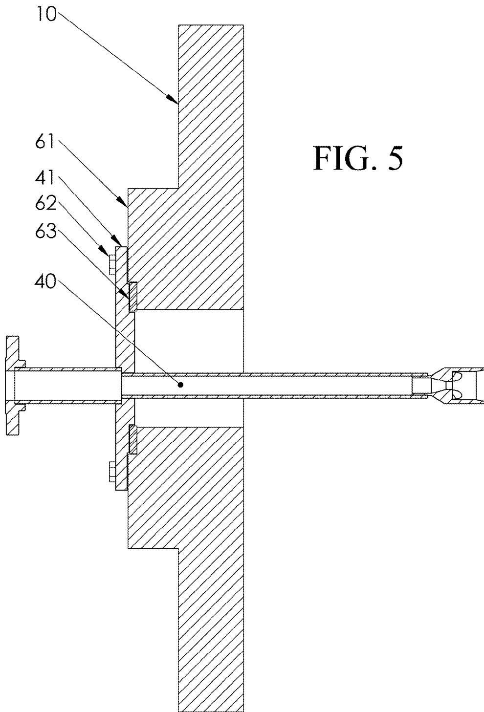
Section View
