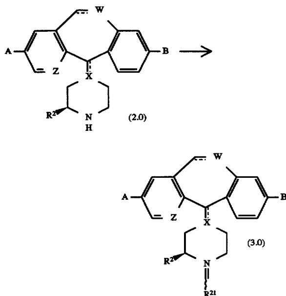
Reaction Scheme 2
