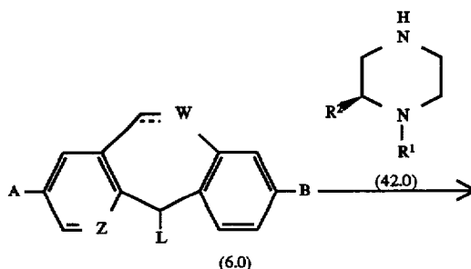
Reaction Scheme 14
