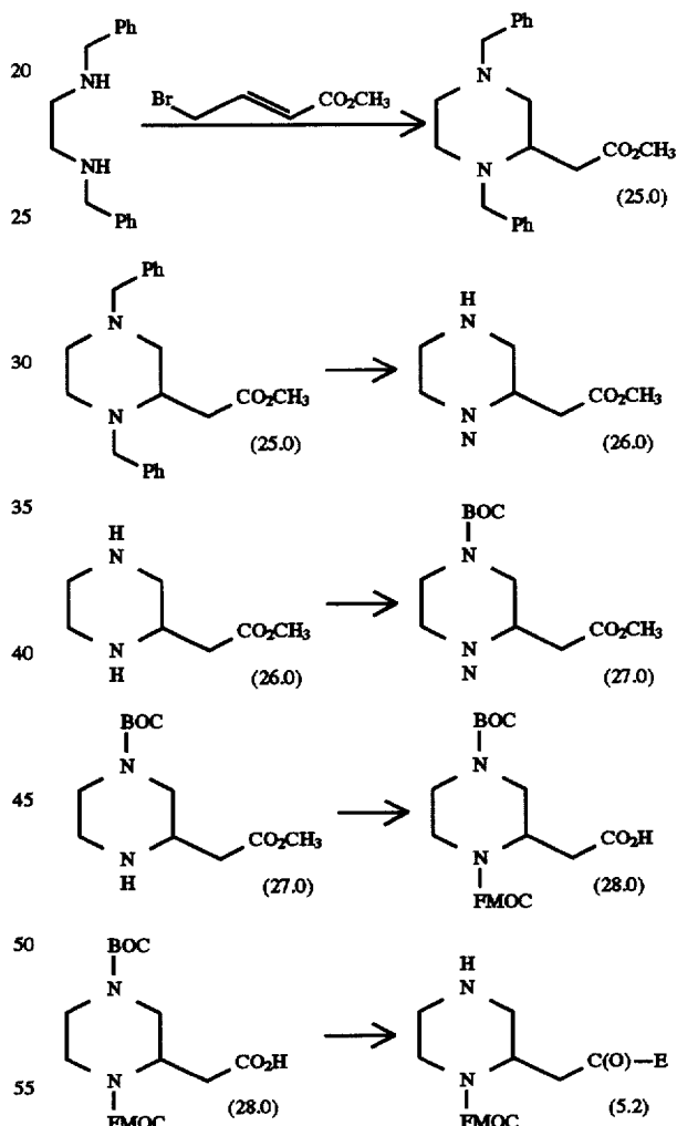
Reaction Scheme 10
