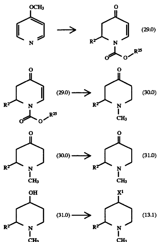
Reaction Scheme 11
