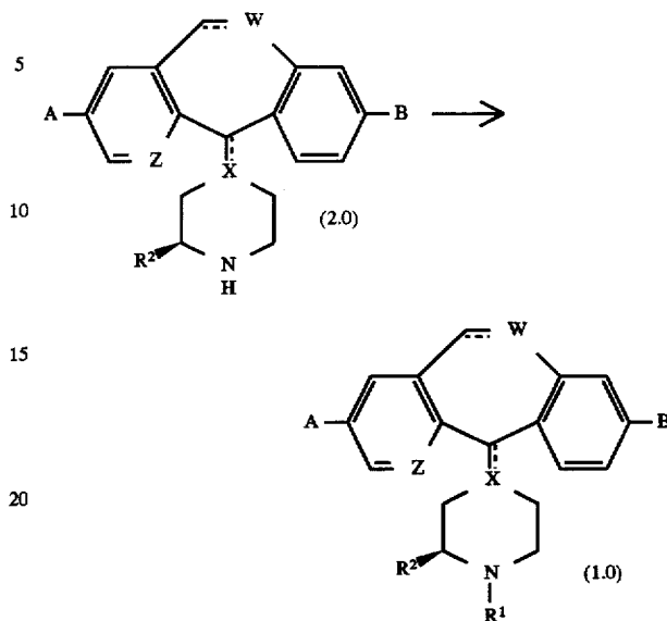
Reaction Scheme 1
