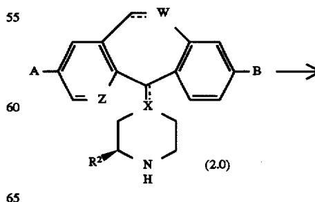
Reaction Scheme 3
