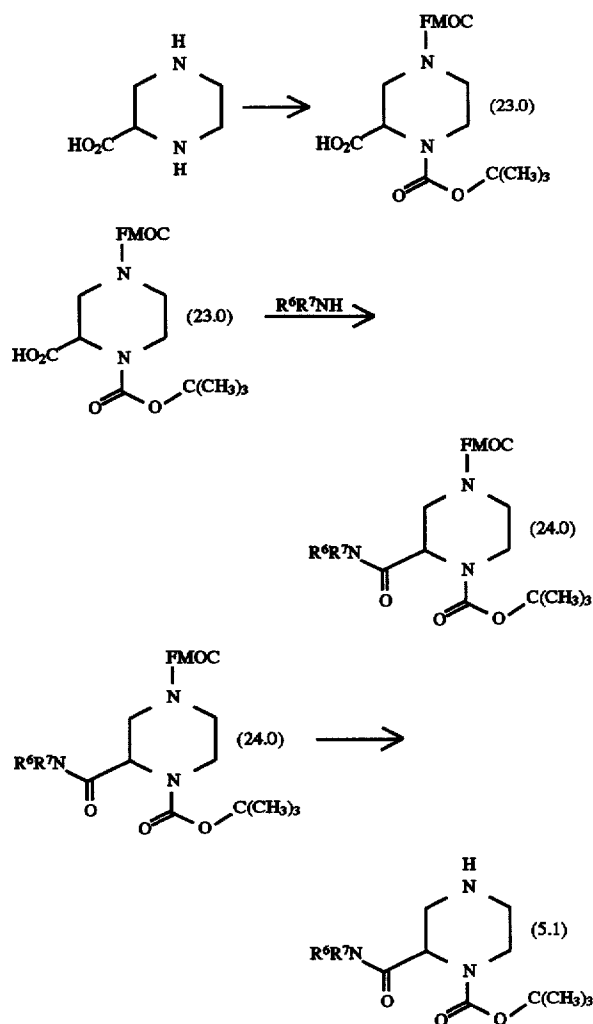
Reaction Scheme 9
