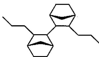
RACEMIC BODY
