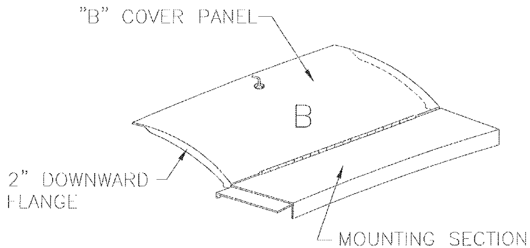
FIGURE 3 PRIOR ART "A" AND "B" COVER PANELS
