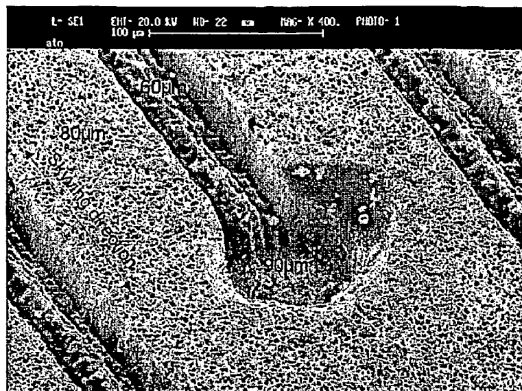
SEM – Detail of hole trench intersection
