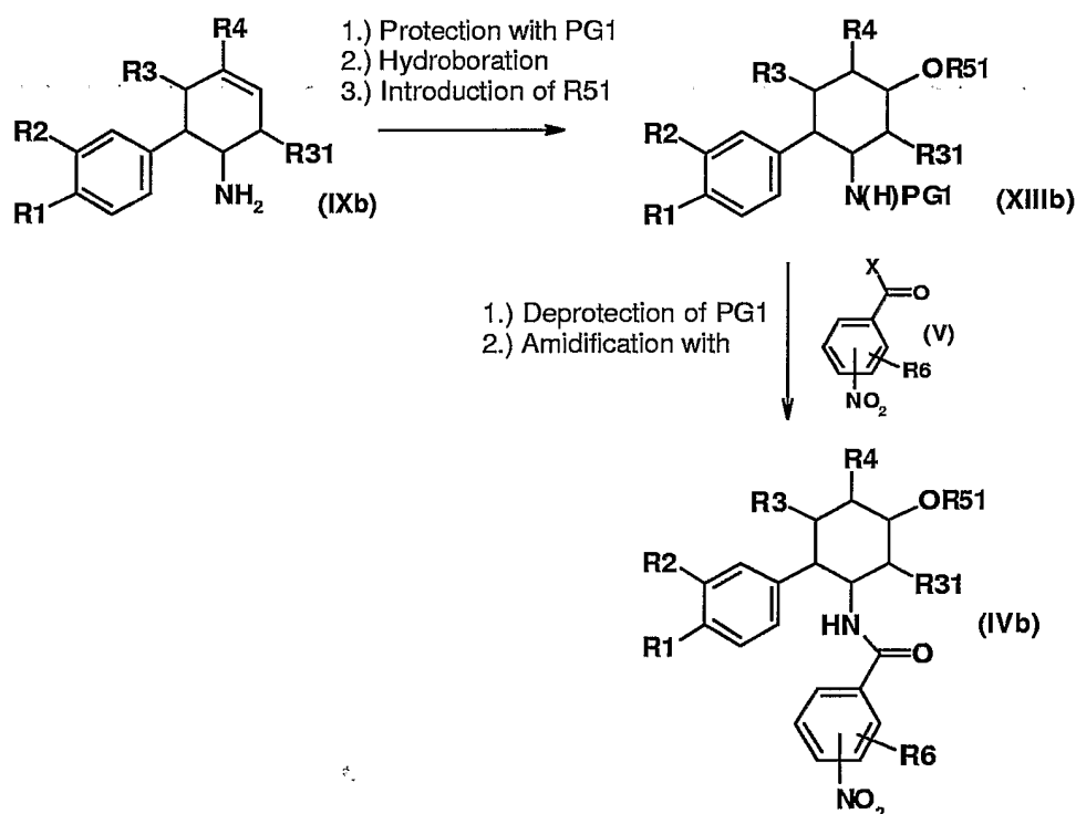
Reaction scheme 7:
