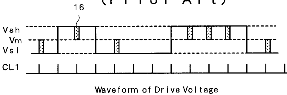
FIG. 14 (Prior Art)
