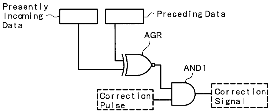
FIG. 13 (Prior Art)
