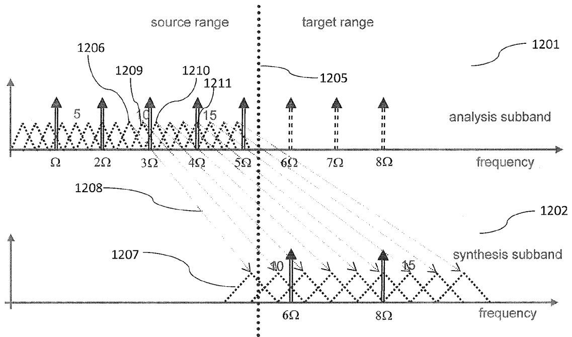
Fig. 12 - PRIOR ART
