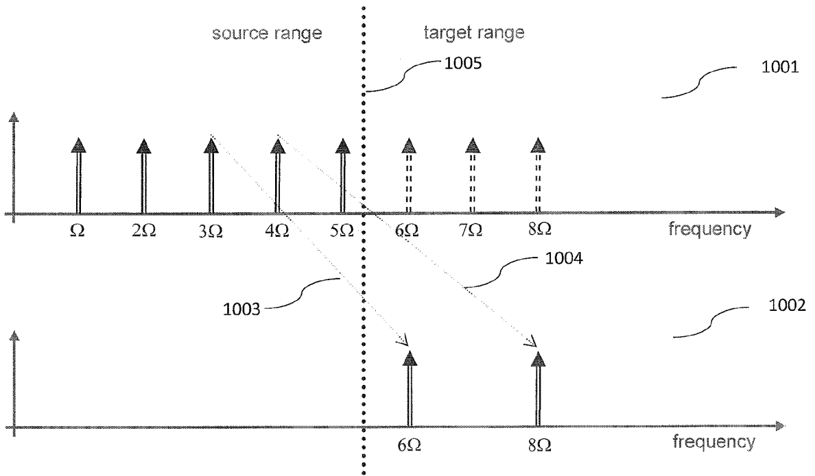
Fig. 10 - PRIOR ART
