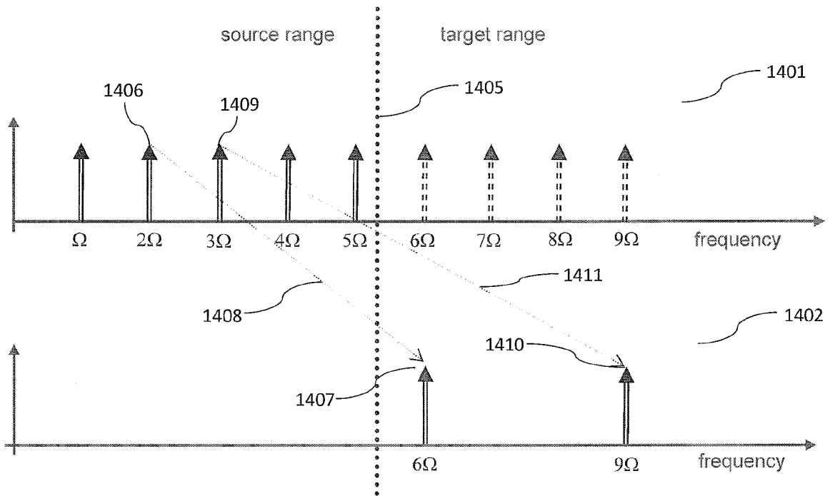
Fig. 14 - PRIOR ART
