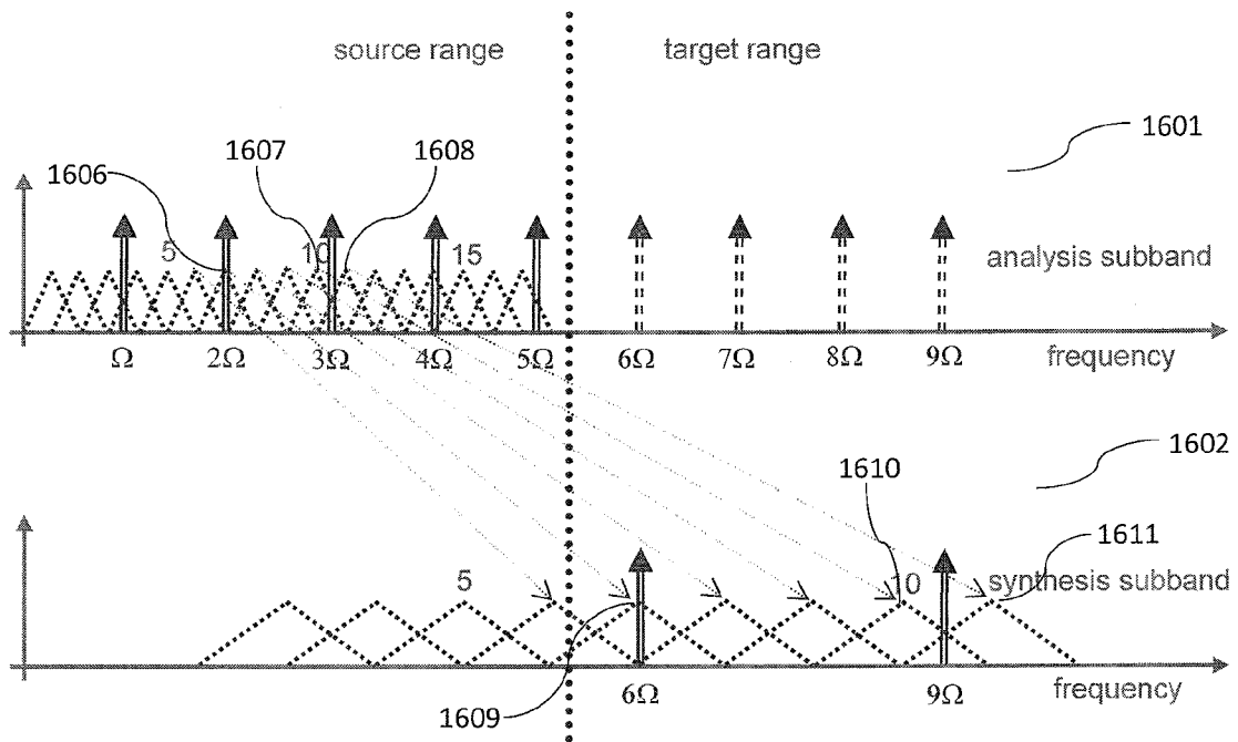
Fig. 16 - PRIOR ART
