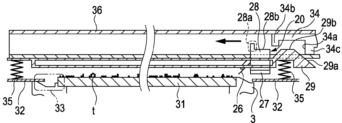
FIG. 5A HOME POSITION
