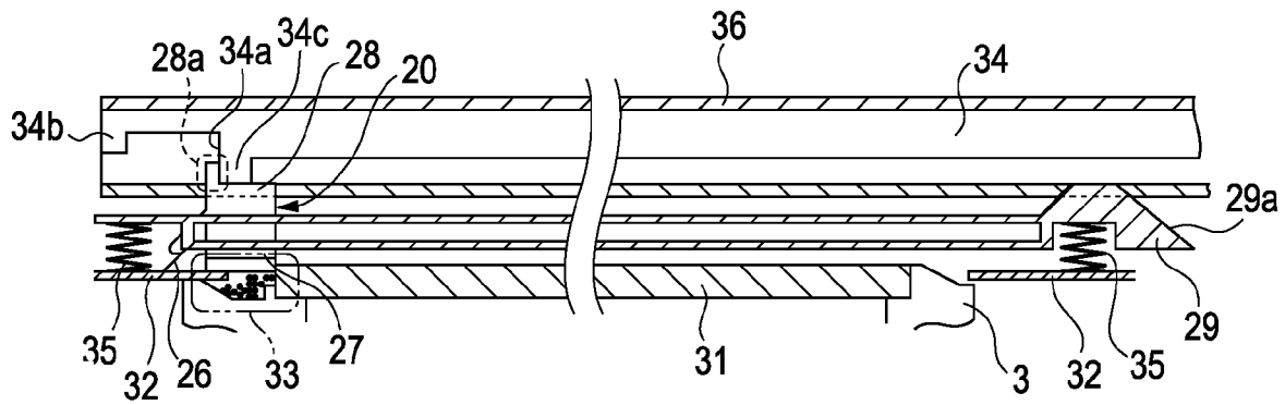
FIG. 6A END OF CLEANING
