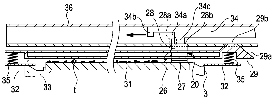
FIG. 5B DURING CLEANING
