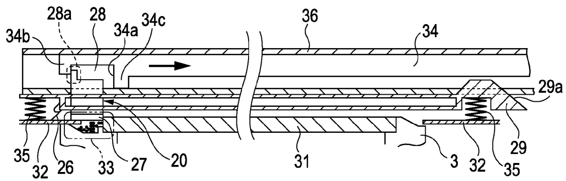
FIG. 6B RETURN TO HOME POSITION
