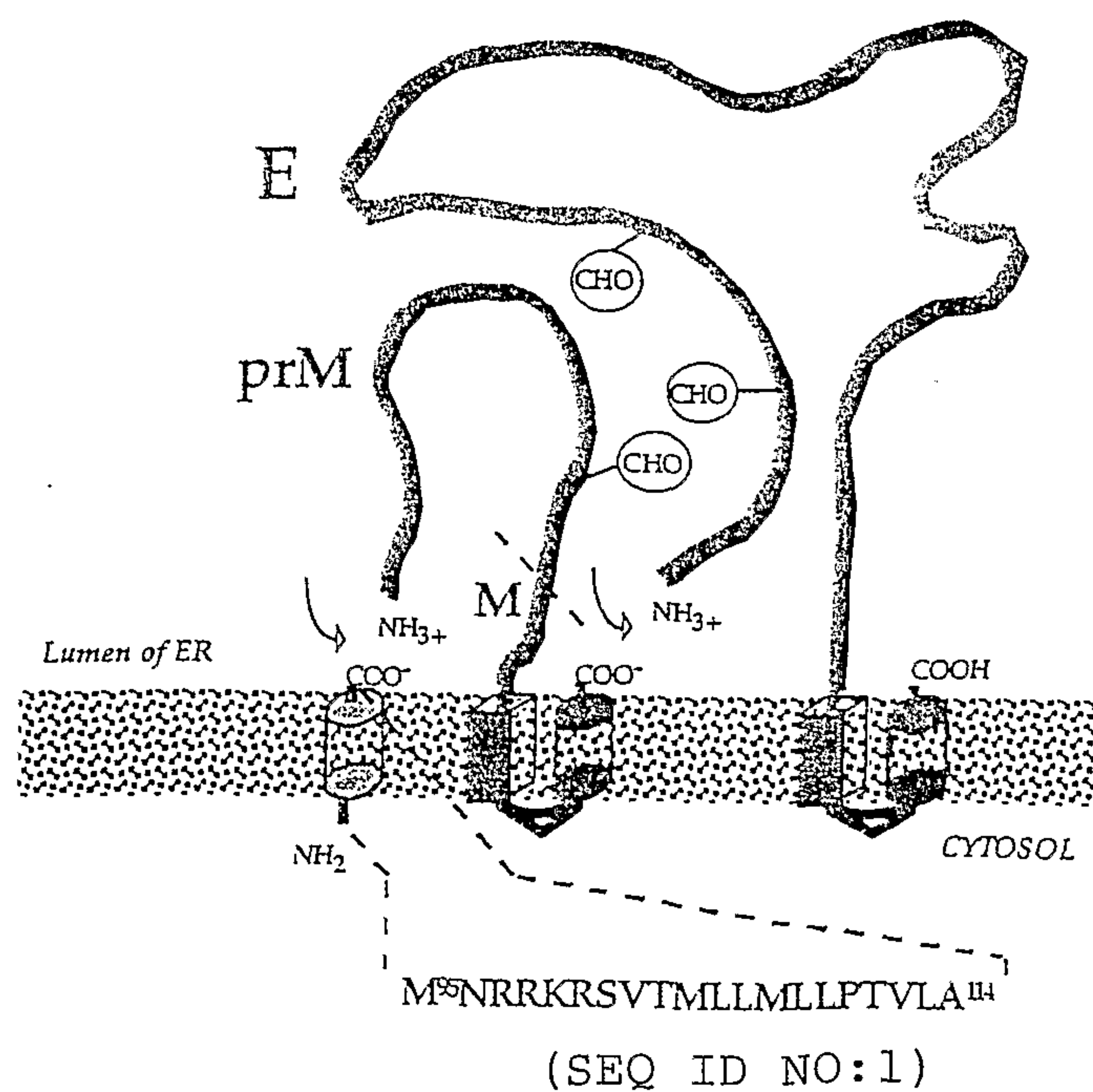
A. Schematic representation of DEN polyprotein maturation.
