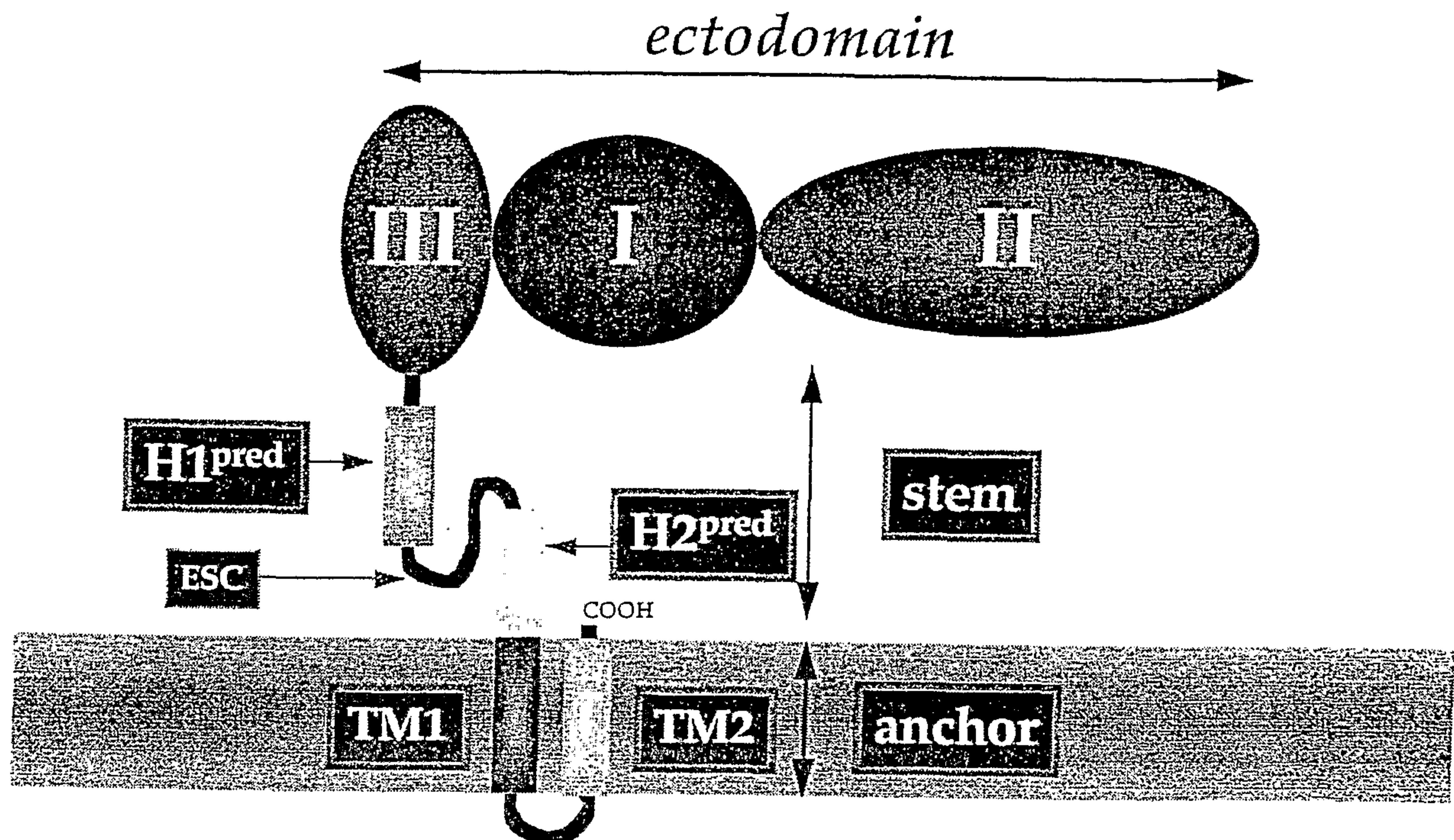
A. Schematic representation of the E protein structure
