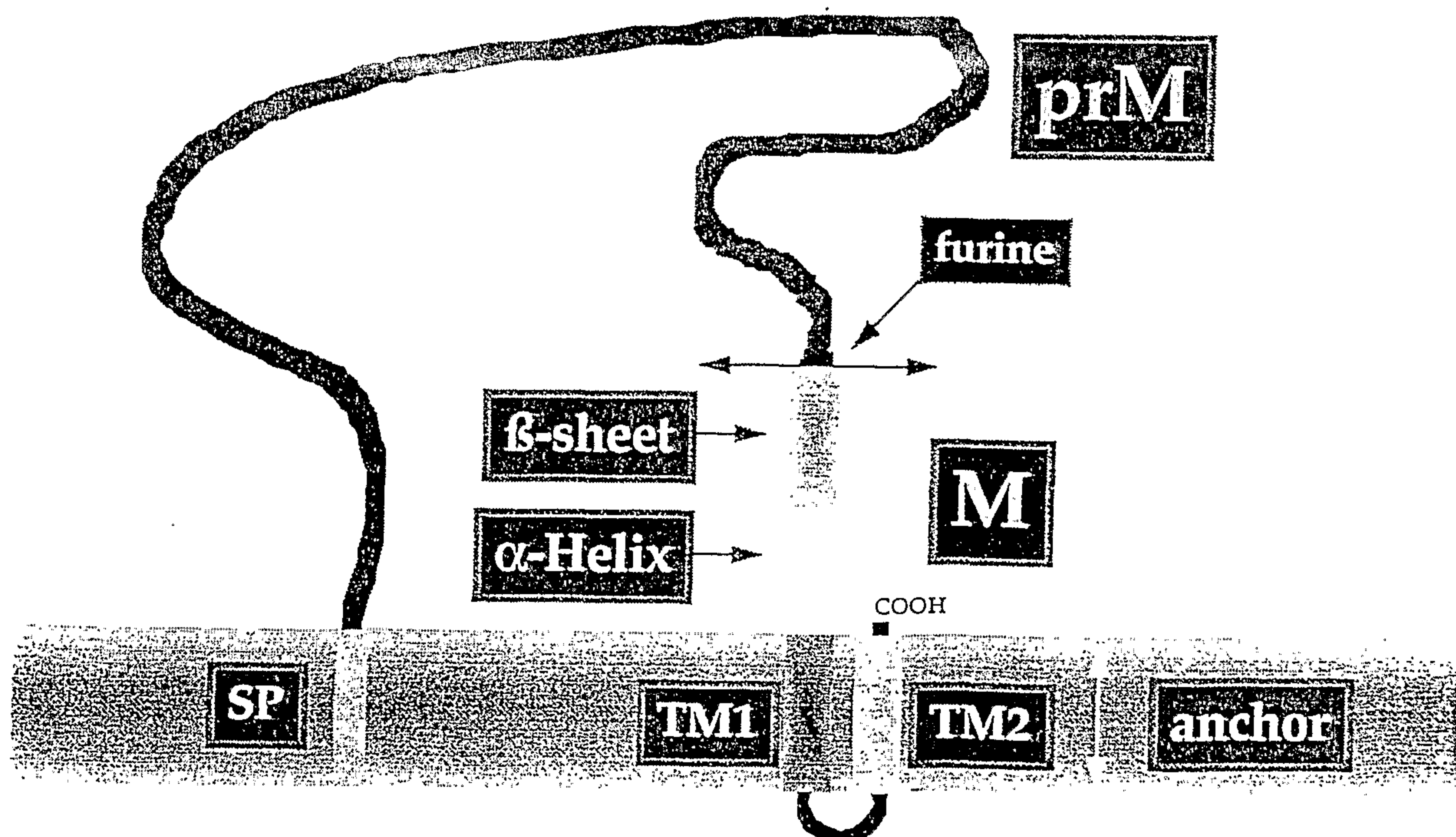
B. Schematic representation of the prM protein structure
