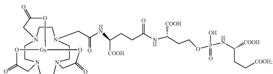
gallium 2,2',2''-(10-(2-(((1S)-1-carboxy-4-(((1S)-1-carboxy-3-(((S)-1,3-dicarboxypropyl)amino)(hydroxyl)phosphoryl)oxy)propyl)amino)-4-oxobutyl)amino)-2-oxoethyl)-1,4,7,10-tetraazacyclododecane-1,4,7-triyl)triacetate
