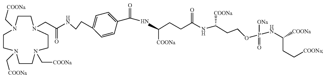
sodium (S)-2-(((S)-3-carboxylato-3-((S)-4-carboxylato-4-(4-(2-(2-(4,7,10-tris(carboxylatomethyl)-1,4,7,10-tetraazacyclododecan-1-yl)acetamido)ethyl)benzamido)butanamido)propoxy)oxidophosphoryl)amino)pentanedioate
