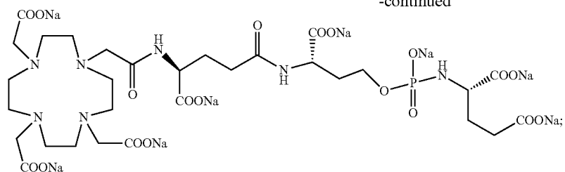
sodium (S)-2-(((S)-3-carboxylato-3-((S)-4-carboxylato-4-(2-(4,7,10-tris(carboxylatomethyl)-1,4,7,10-tetraazacyclododecan-1-yl)acetamido)butanamido)propoxy)oxidophosphoryl)amino)pentanedioate
