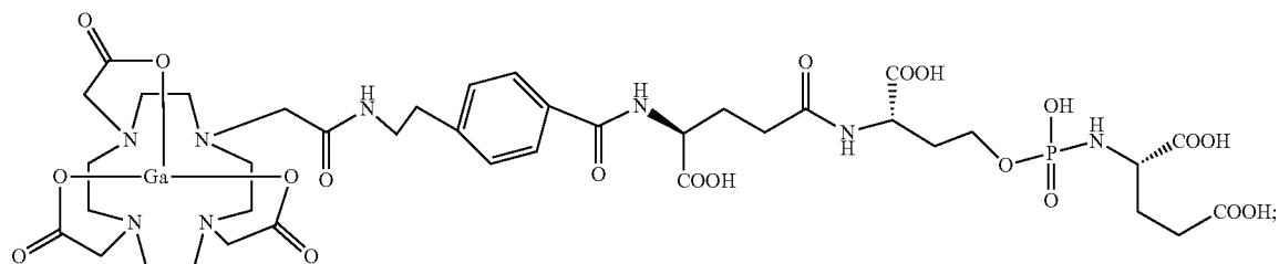
gallium 2,2',2''-(10-(2-((4-(((1S)-1-carboxy-4-(((1S)-1-carboxy-3-(((S)-1,3-dicarboxypropyl)amino)(hydroxyl)phosphoryl)oxy)propyl)amino)-4-oxobutyl)carbamoyl)phenethyl)amino)-2-oxoethyl)-1,4,7,10-tetraazacyclododecane-1,4,7-triyl)triacetate
