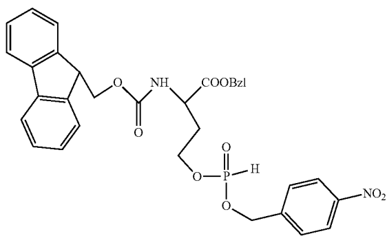
1 MW630.58
