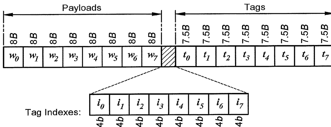
Cache line compression in DRAM
