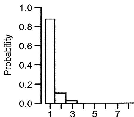
Unique tags per DRAM transfer for gcc
