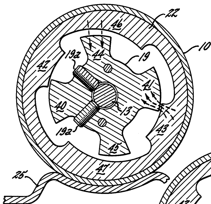
FIG. 3. 0° SHAFT POSITION
