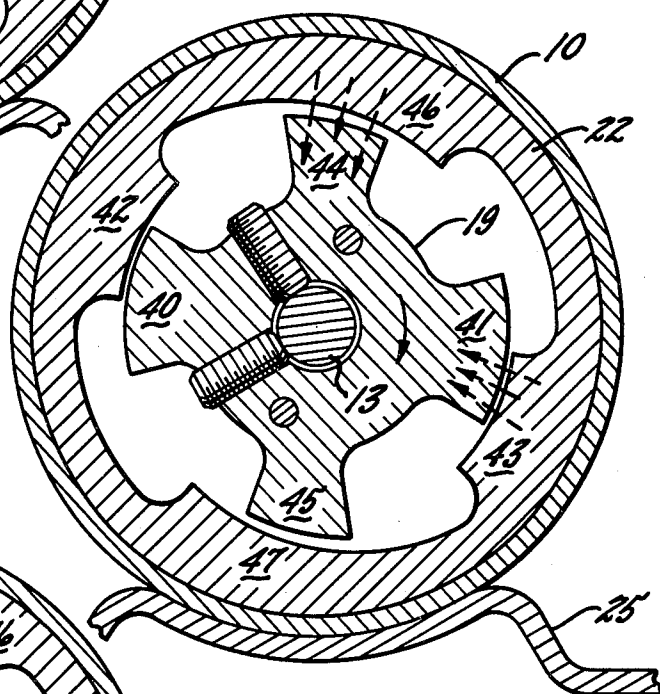
FIG. 4. 15° SHAFT POSITION
