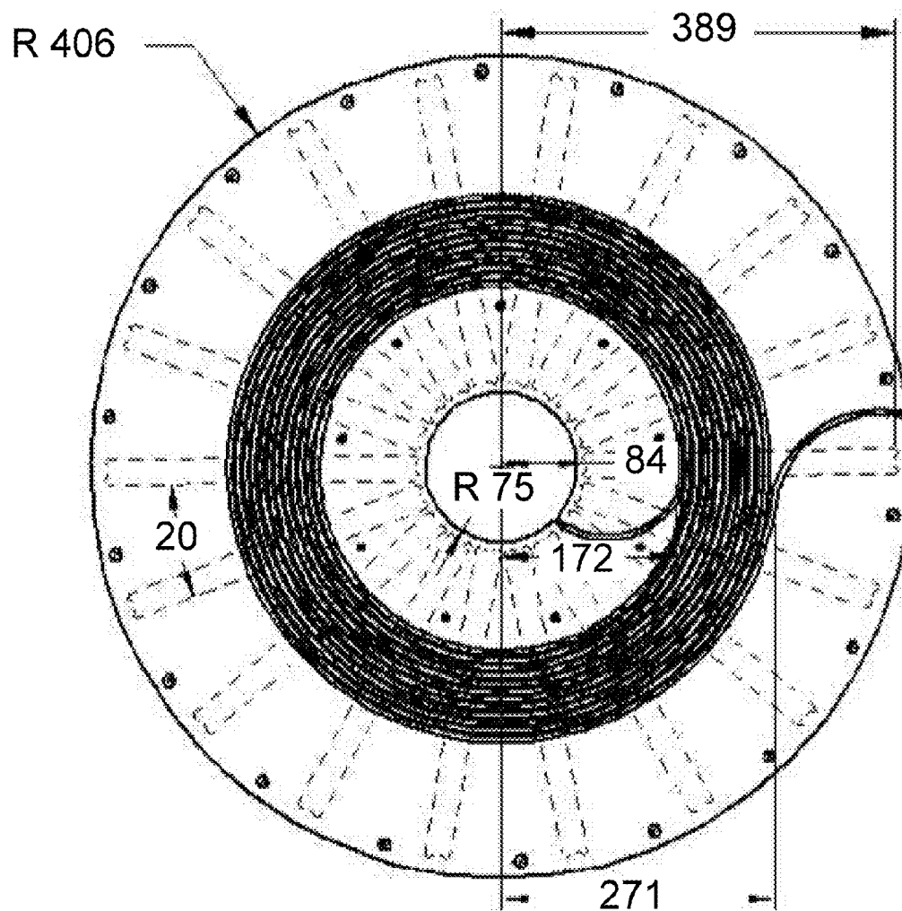
Circular pad structure and dimension (Top View)
