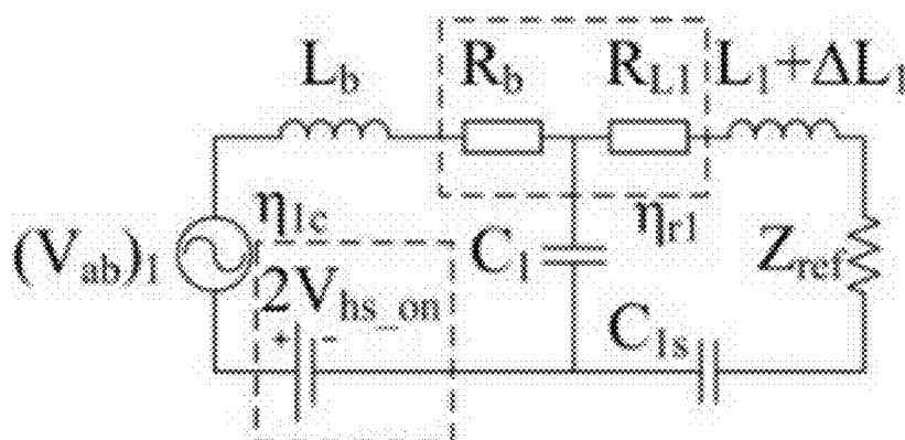
Equivalent efficiency model circuit diagram of primary LCL converter (see also Figure 11)
