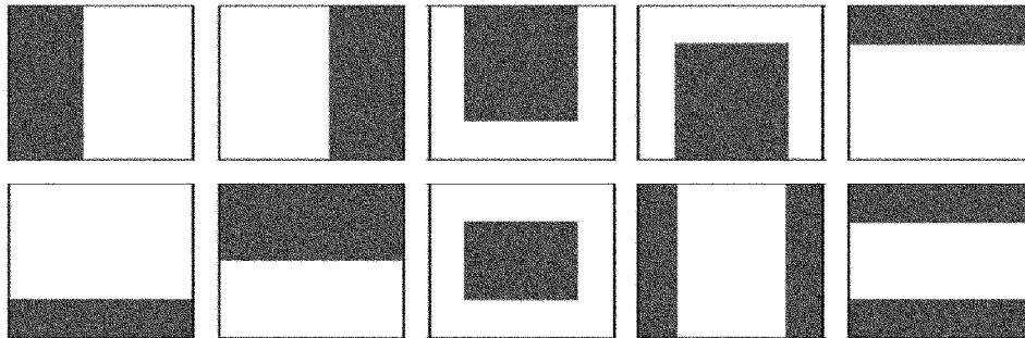
Ten different types of Haar-like features for pedestrian detection
