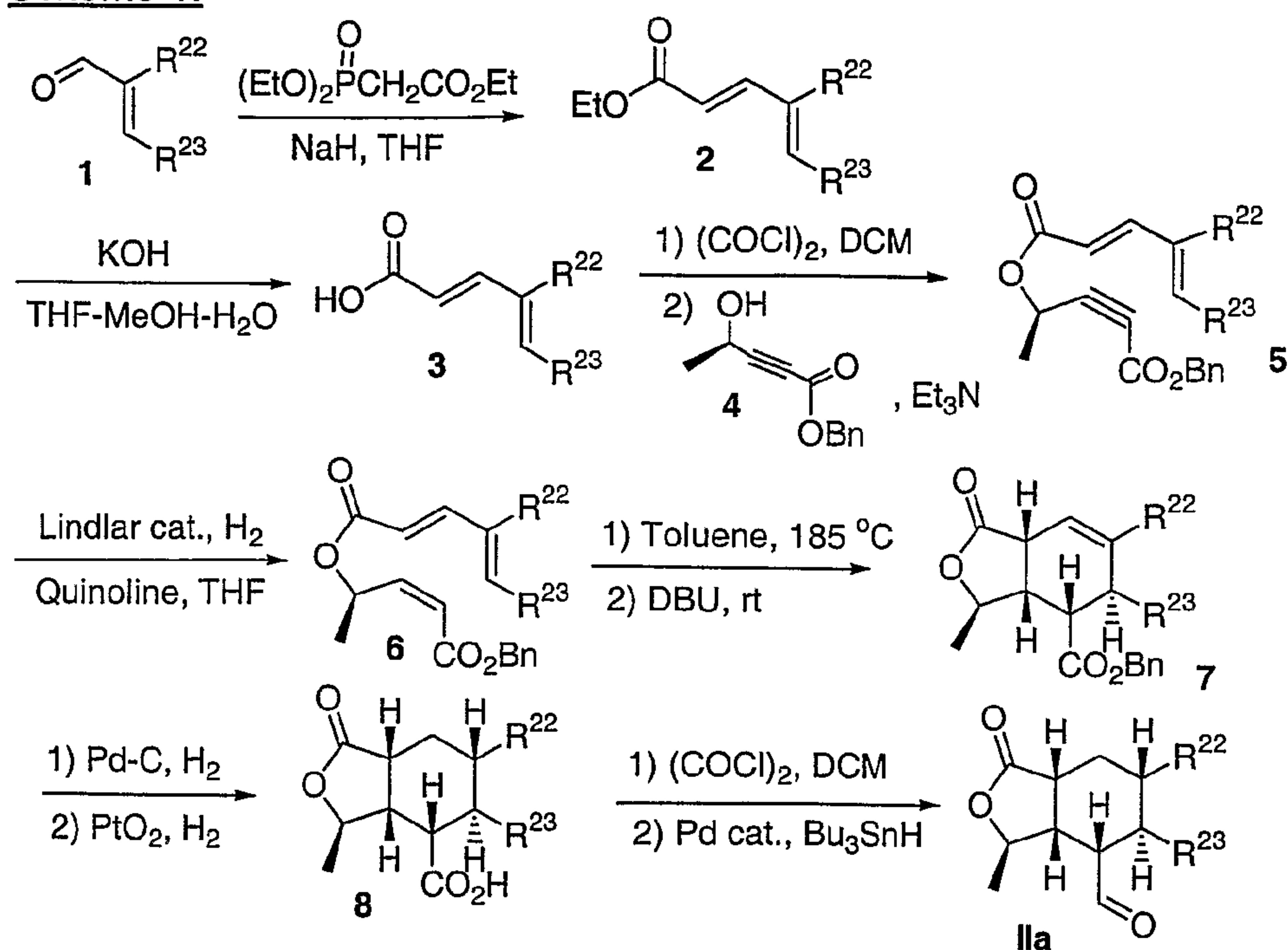
Scheme 1:
