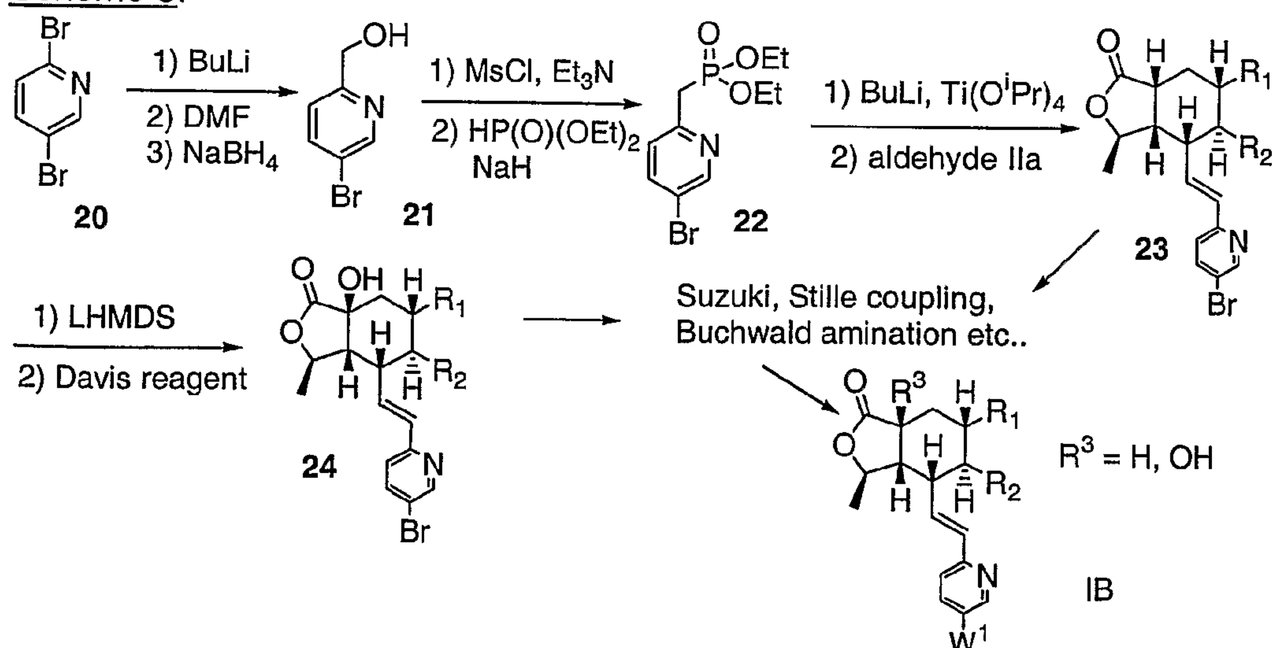
Scheme 5:
