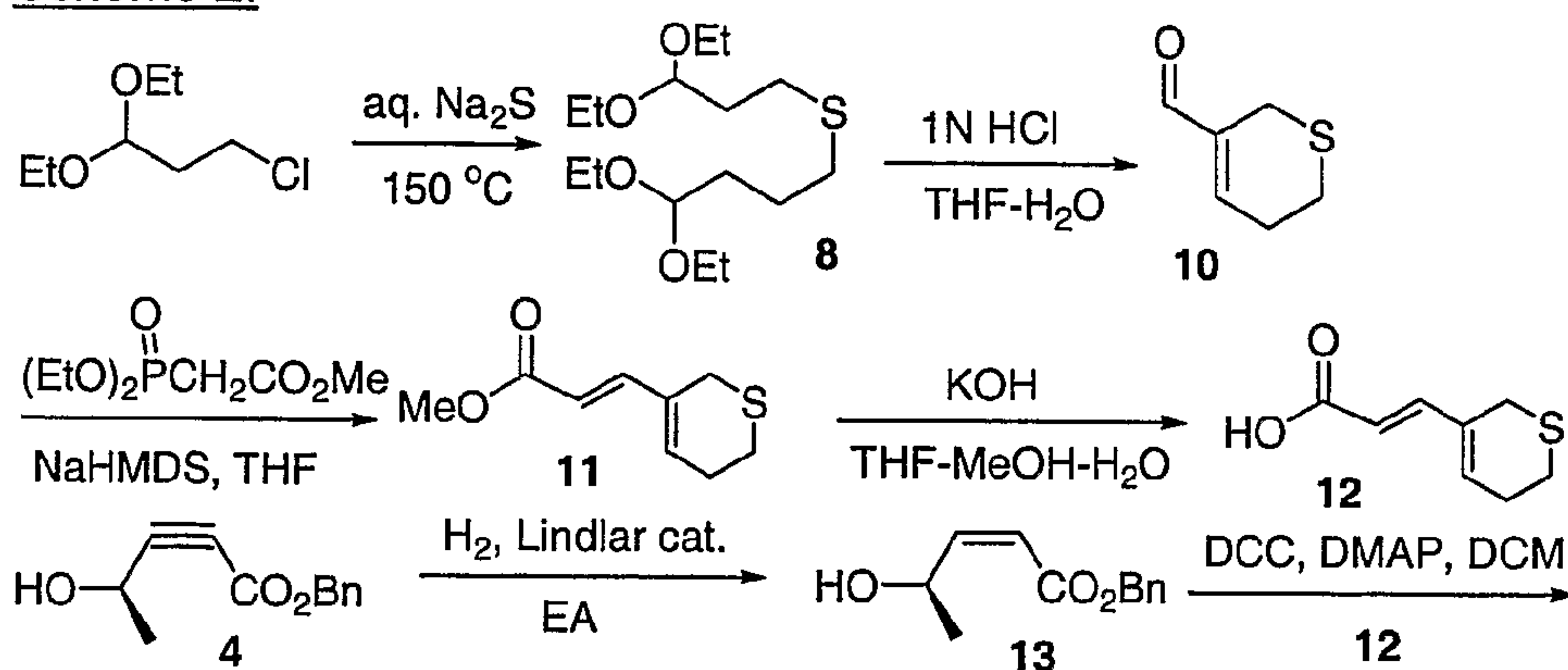
Scheme 2:
