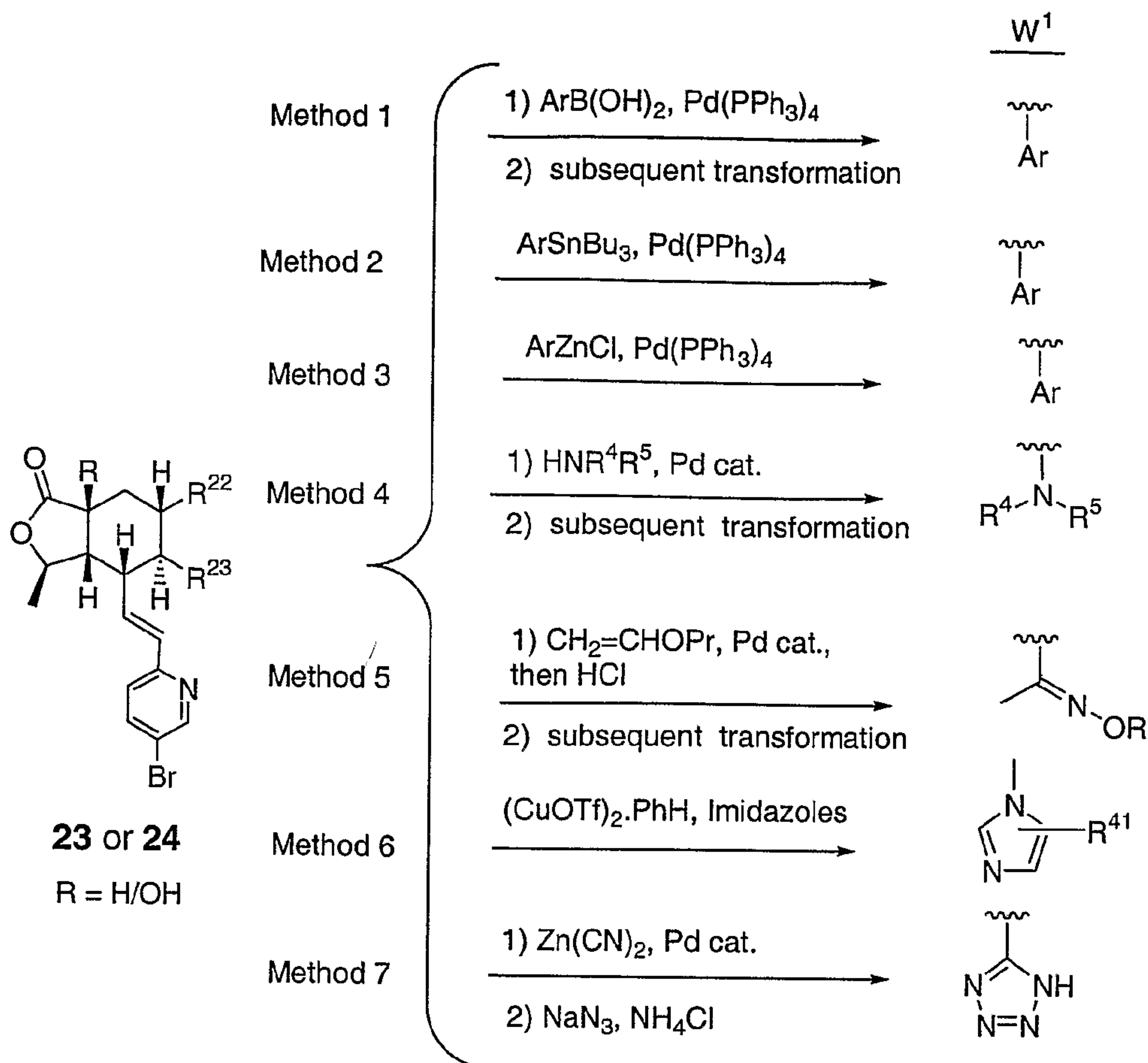
Scheme 6:
