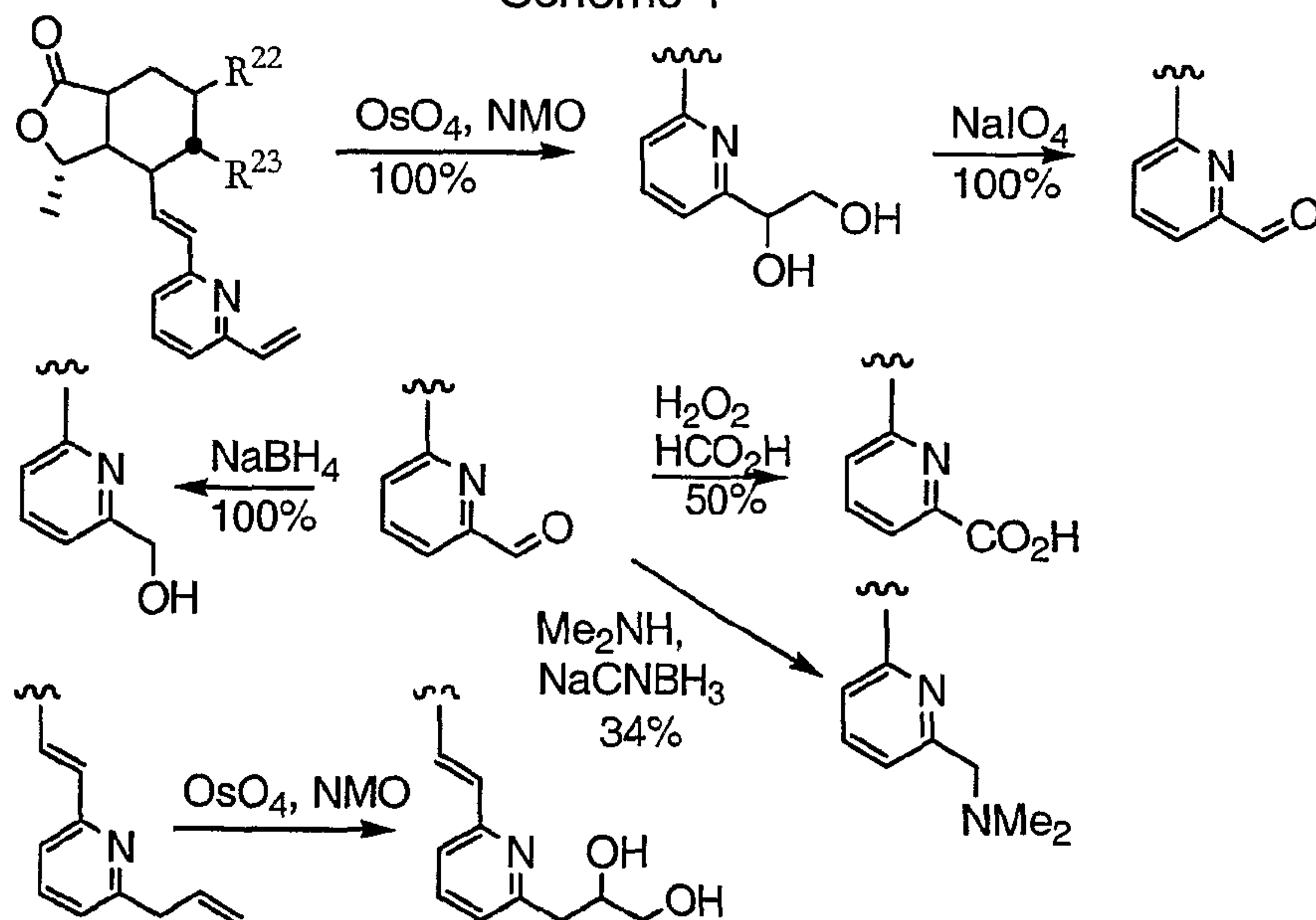
Scheme 4
