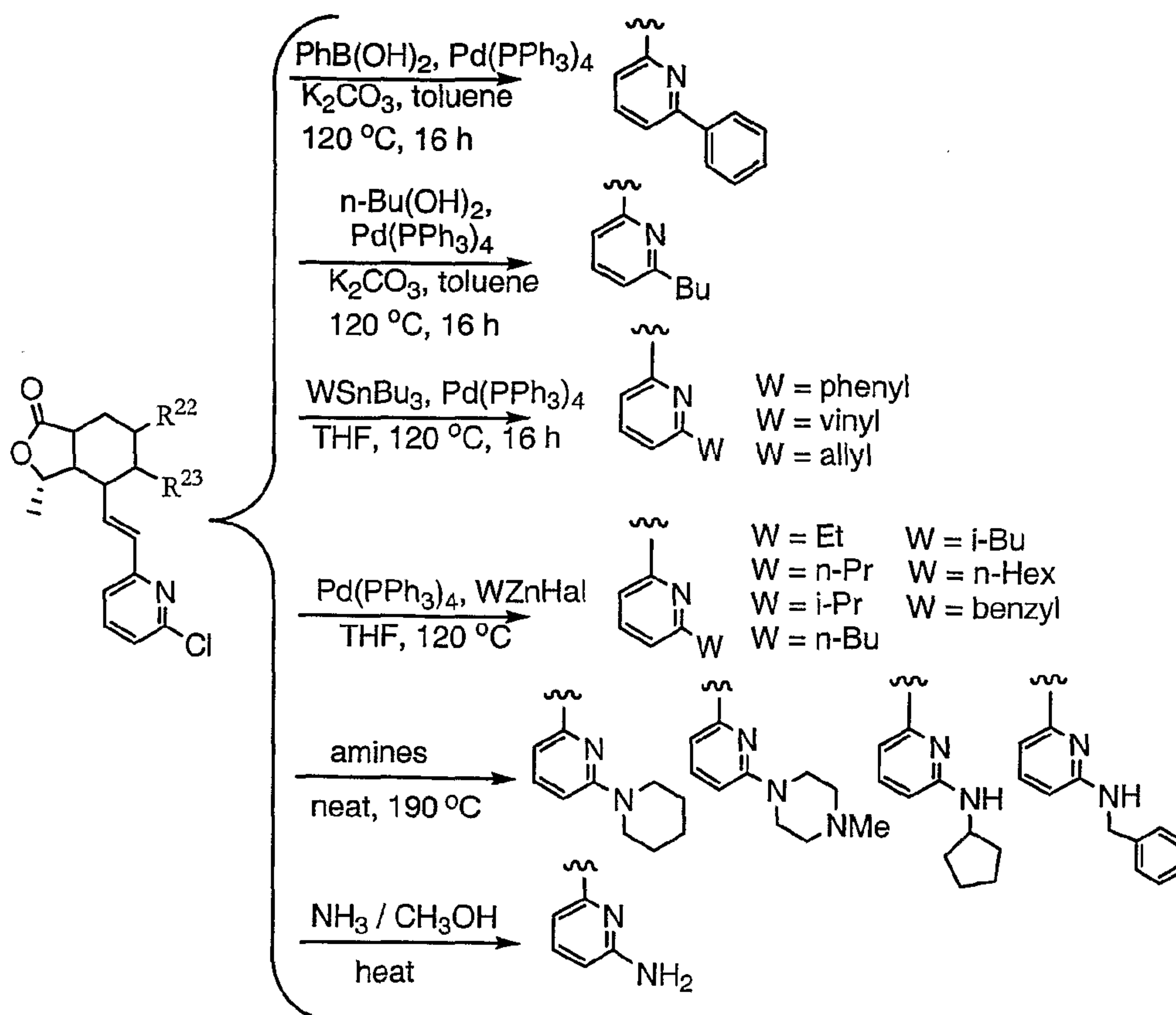
Scheme 4
