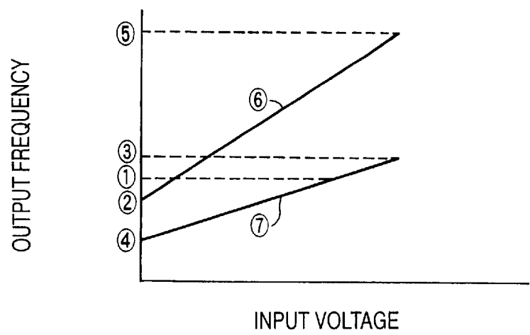
Fig. 3 PRIOR ART
