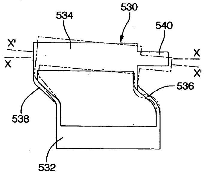
PRIOR ART FIG. 47
