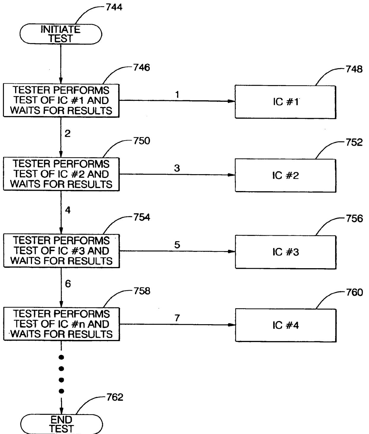
PRIOR ART FIG. 55
